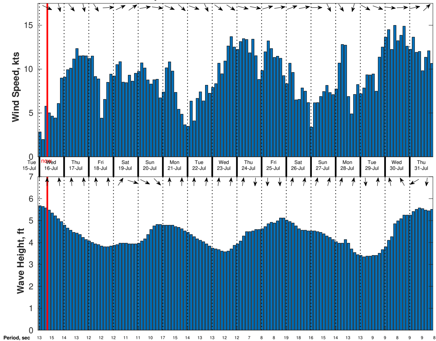
Wind & Wave Forecast for Gyre from 15-Jul-2025 23:00:00 to 31-Jul-2025 23:00:00
