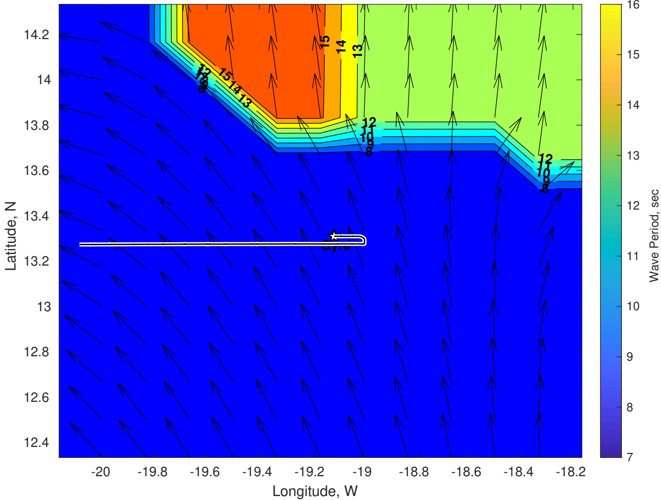
Wave Period (sec) for Gyre at 16-Jul-2025 09:00:00
