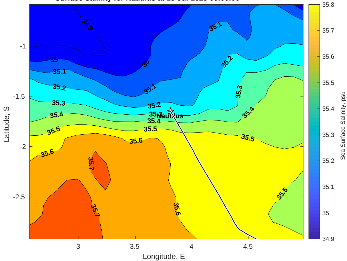
Surface Salinity for Nautilus at 15-Jul-2025 00:00:00
