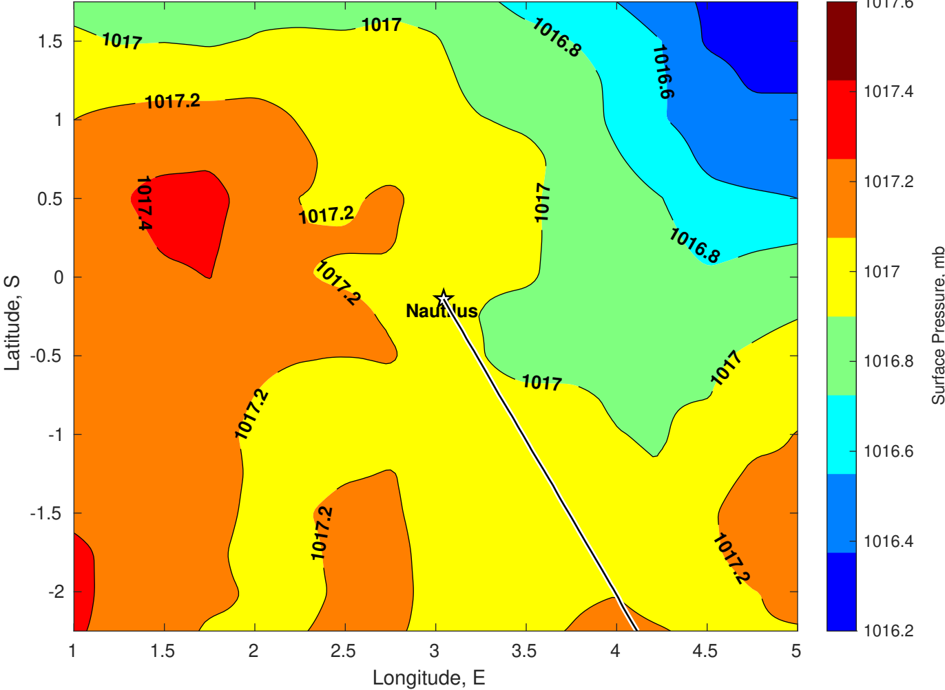
Surface Pressure (mb) for Nautilus at 18-Jul-2025 00:00:00
