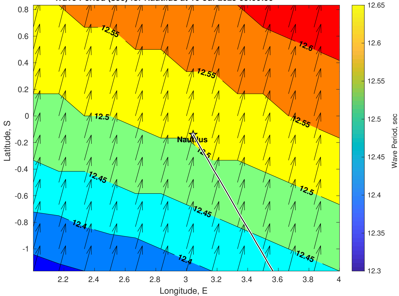
Wave Period (sec) for Nautilus at 16-Jul-2025 09:00:00
