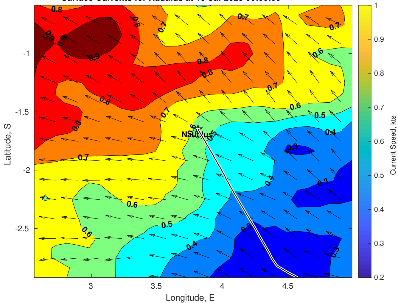
Surface Currents for Nautilus at 15-Jul-2025 00:00:00
