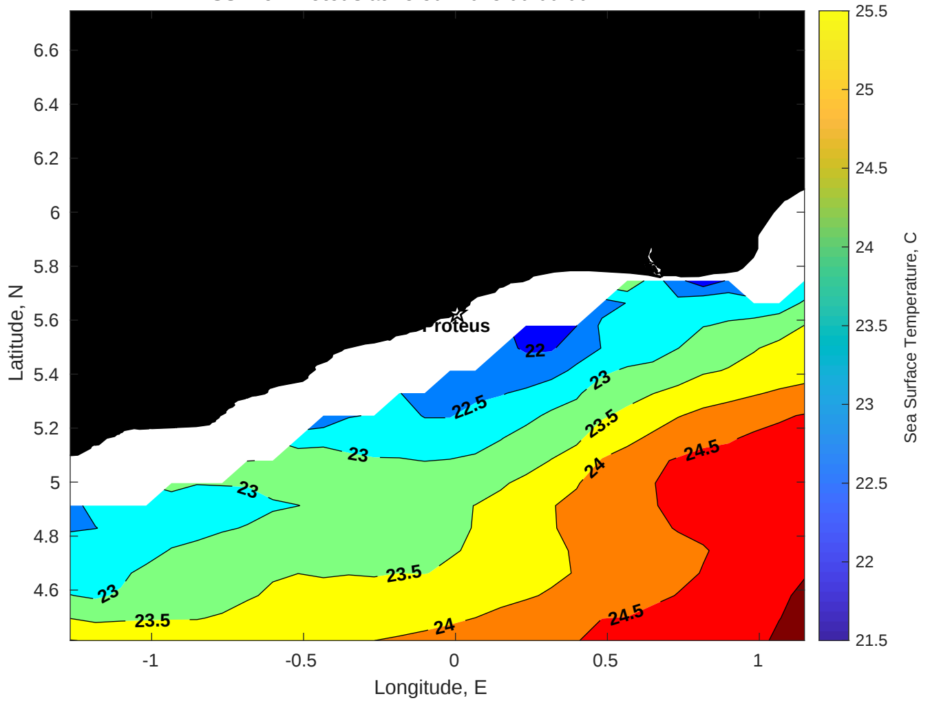
SST for Proteus at 15-Jul-2025 00:00:00
