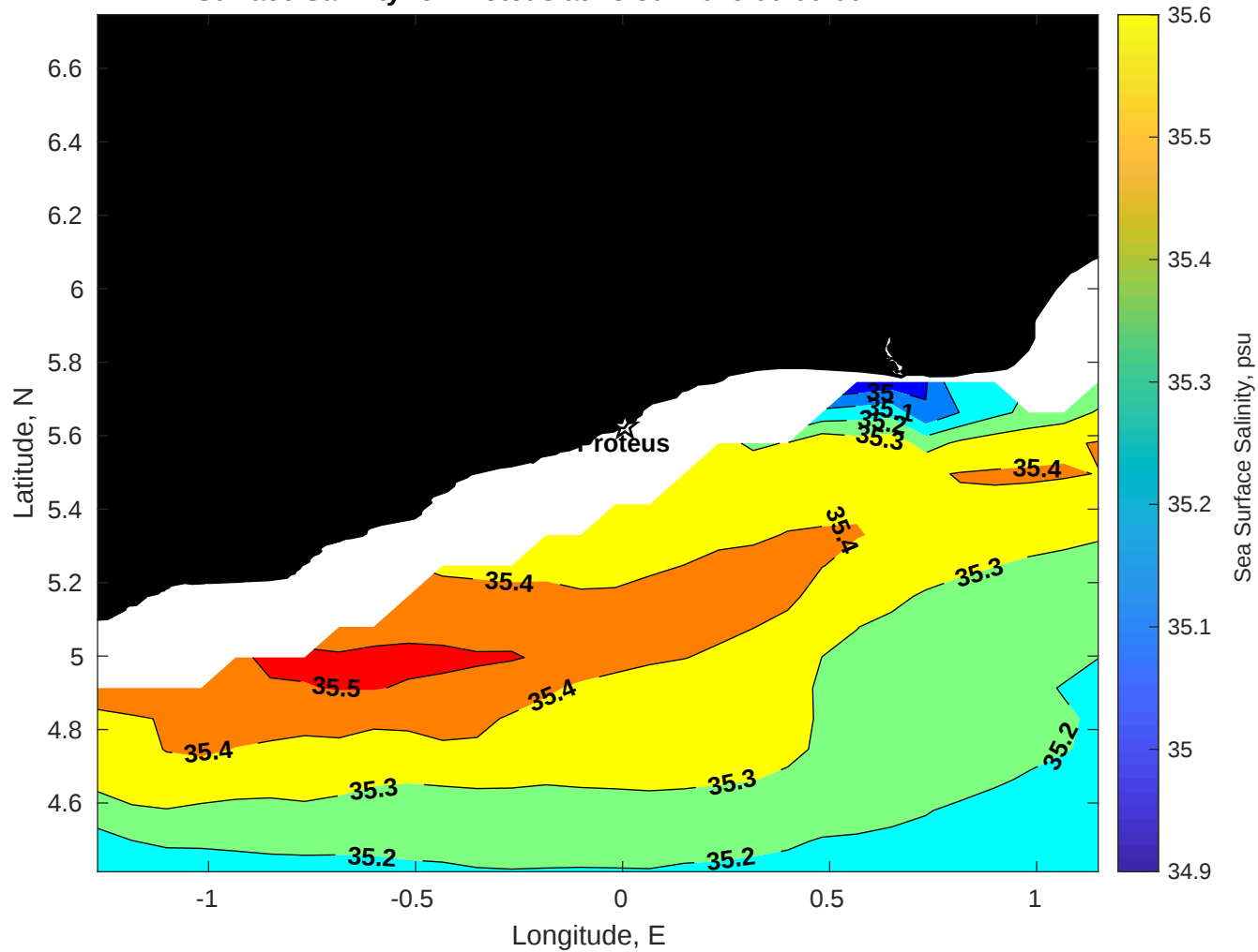
Surface Salinity for Proteus at 15-Jul-2025 00:00:00
