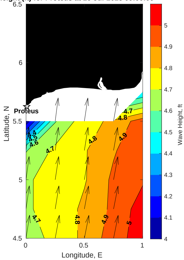
Wave Height (ft) for Proteus at 16-Jul-2025 09:00:00
