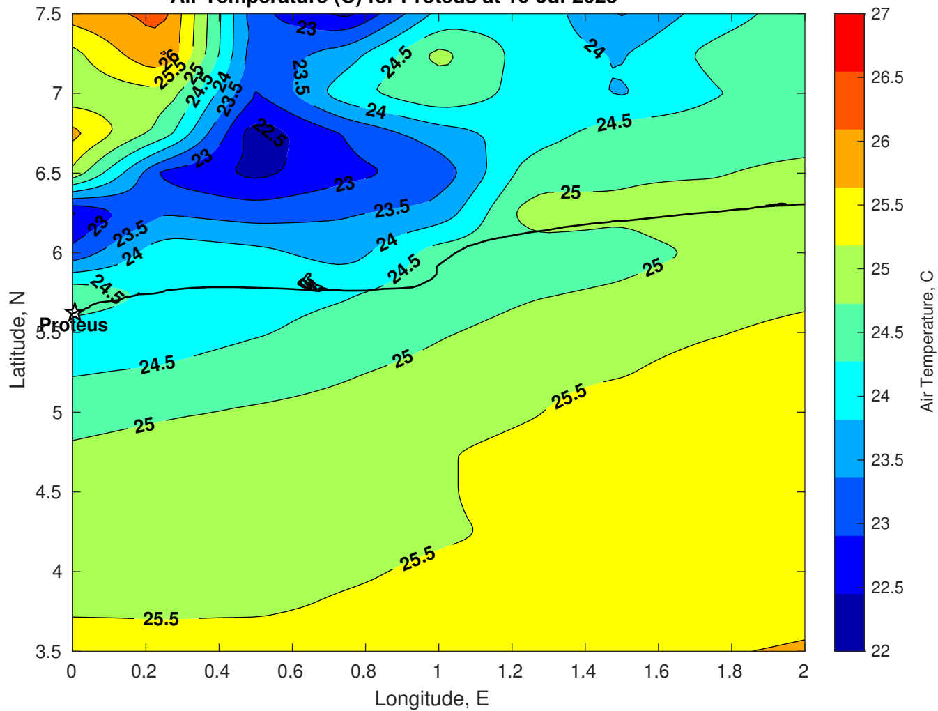
Air Temperature (C) for Proteus at 16-Jul-2025
