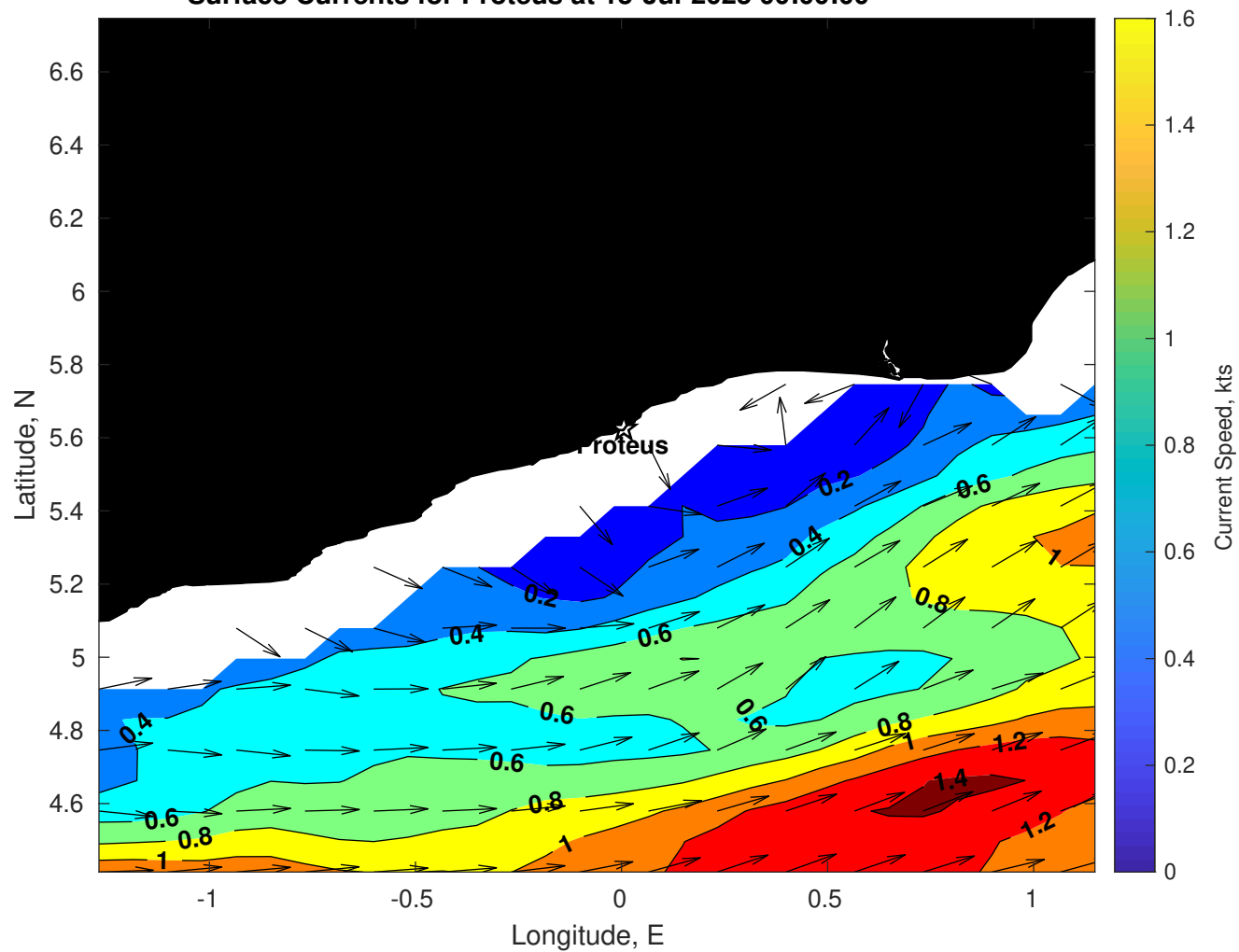
Surface Currents for Proteus at 15-Jul-2025 00:00:00
