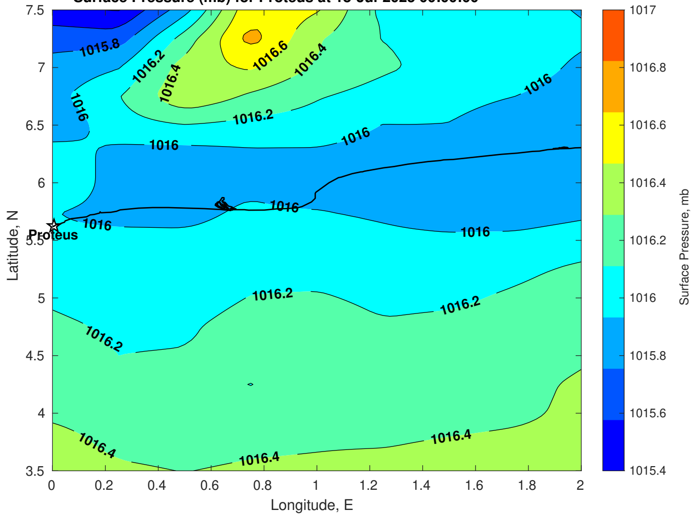
Surface Pressure (mb) for Proteus at 18-Jul-2025 00:00:00
