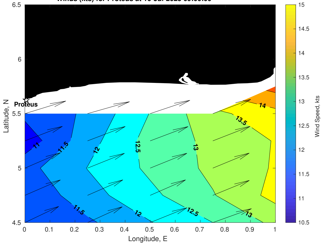
Winds (kts) for Proteus at 16-Jul-2025 09:00:00
