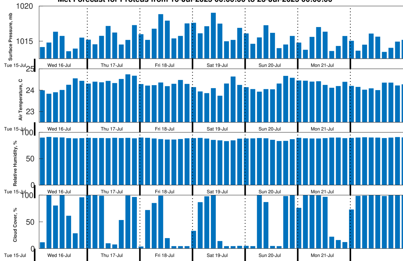
Met Forecast for Proteus from 16-Jul-2025 00:00:00 to 23-Jul-2025 00:00:00
