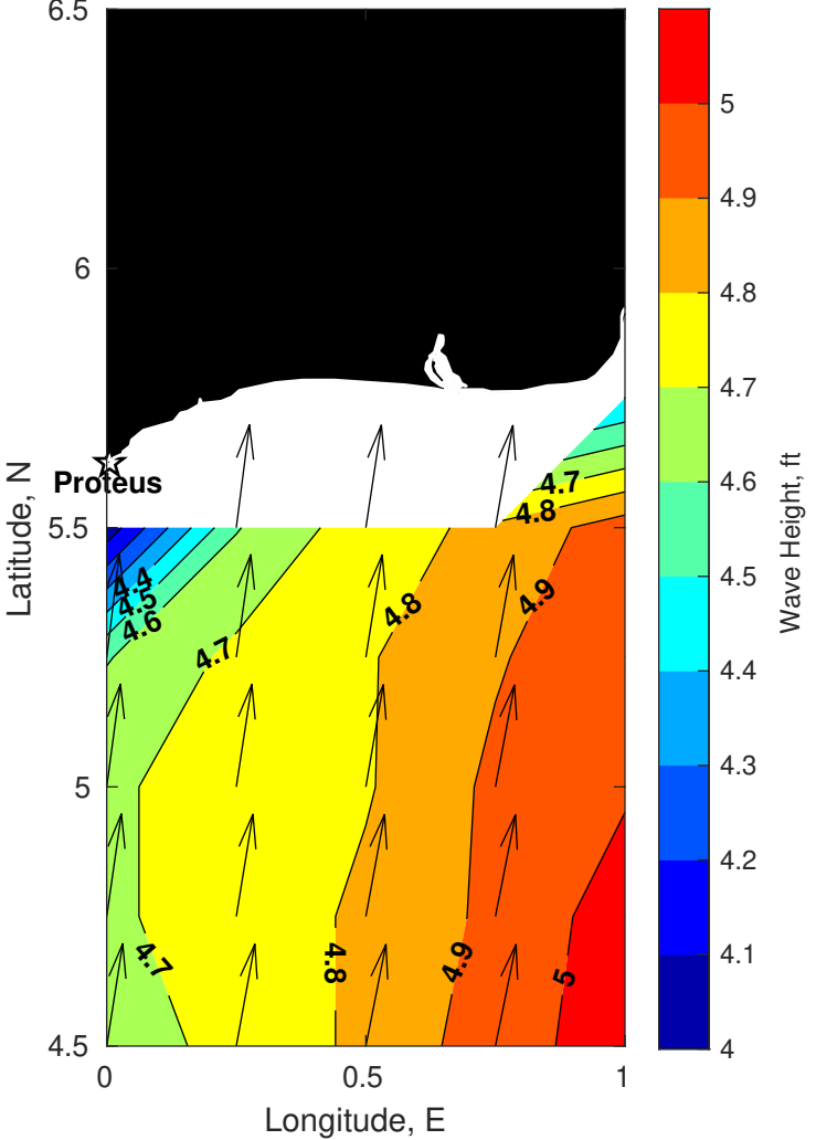
Wave Height (ft) for Proteus at 16-Jul-2025 09:00:00
