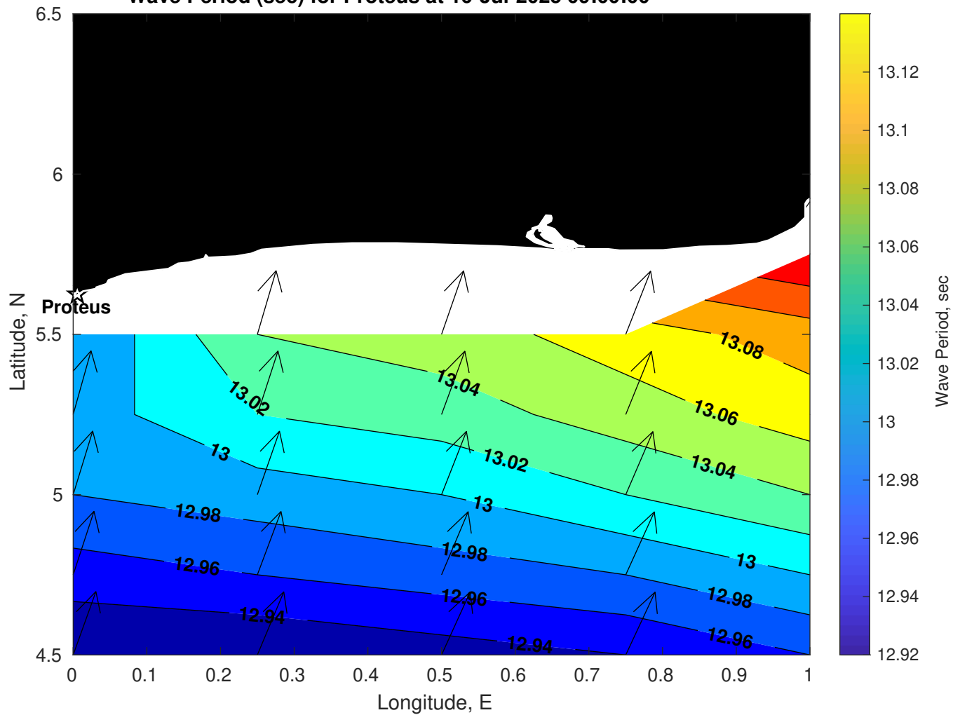
Wave Period (sec) for Proteus at 16-Jul-2025 09:00:00
