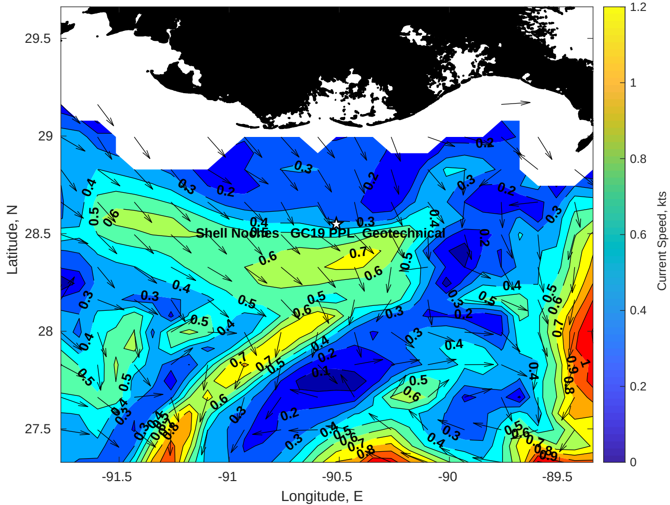
Surface Currents for Shell Noches GC19 PPL Geotechnical at 15-Jul-2025 00:00:00
