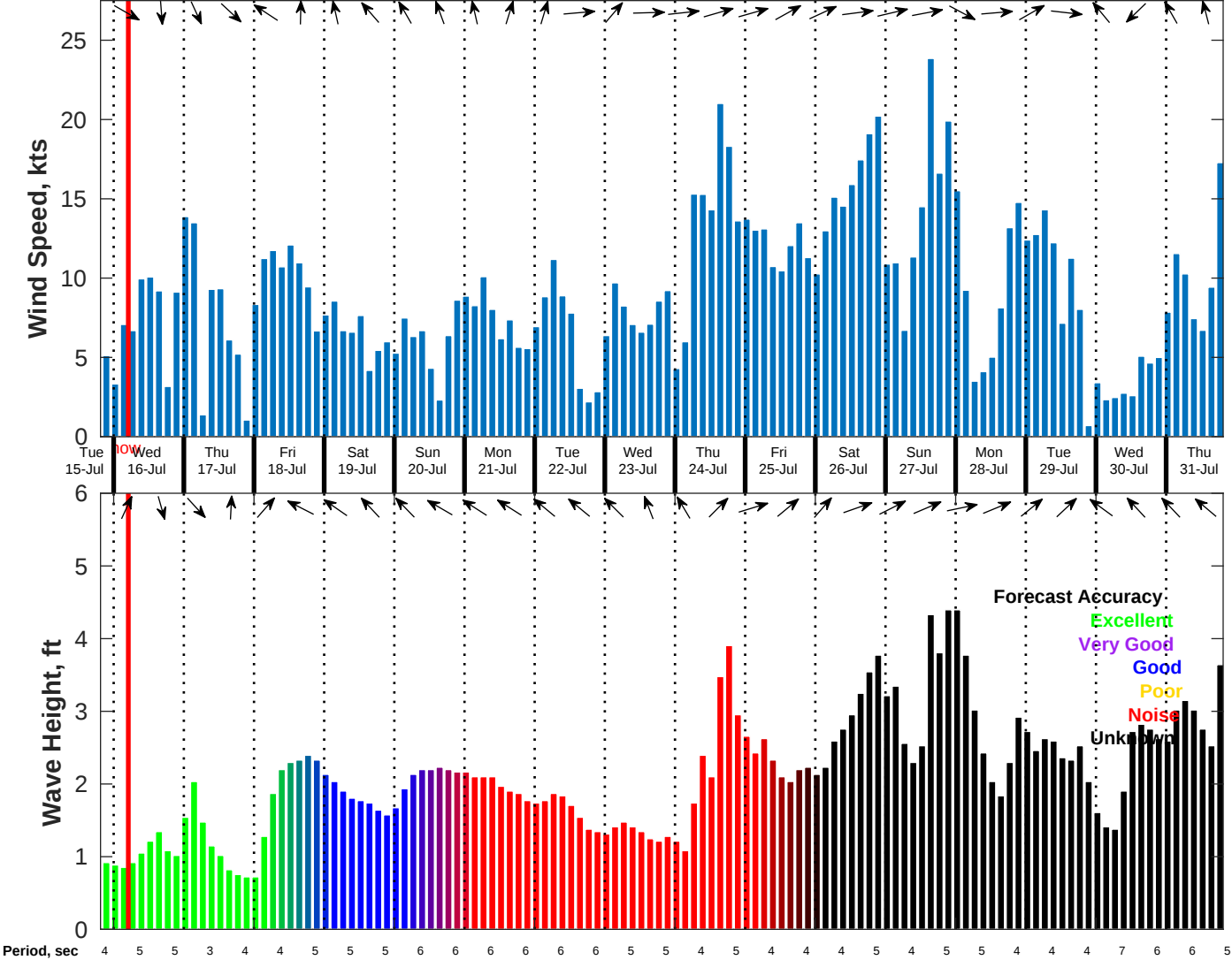
Wind & Wave Forecast for Shell Noches GC19 PPL Geotechnical from 15-Jul-2025 20:00:00 to 31-Jul-2025 20:00:00
