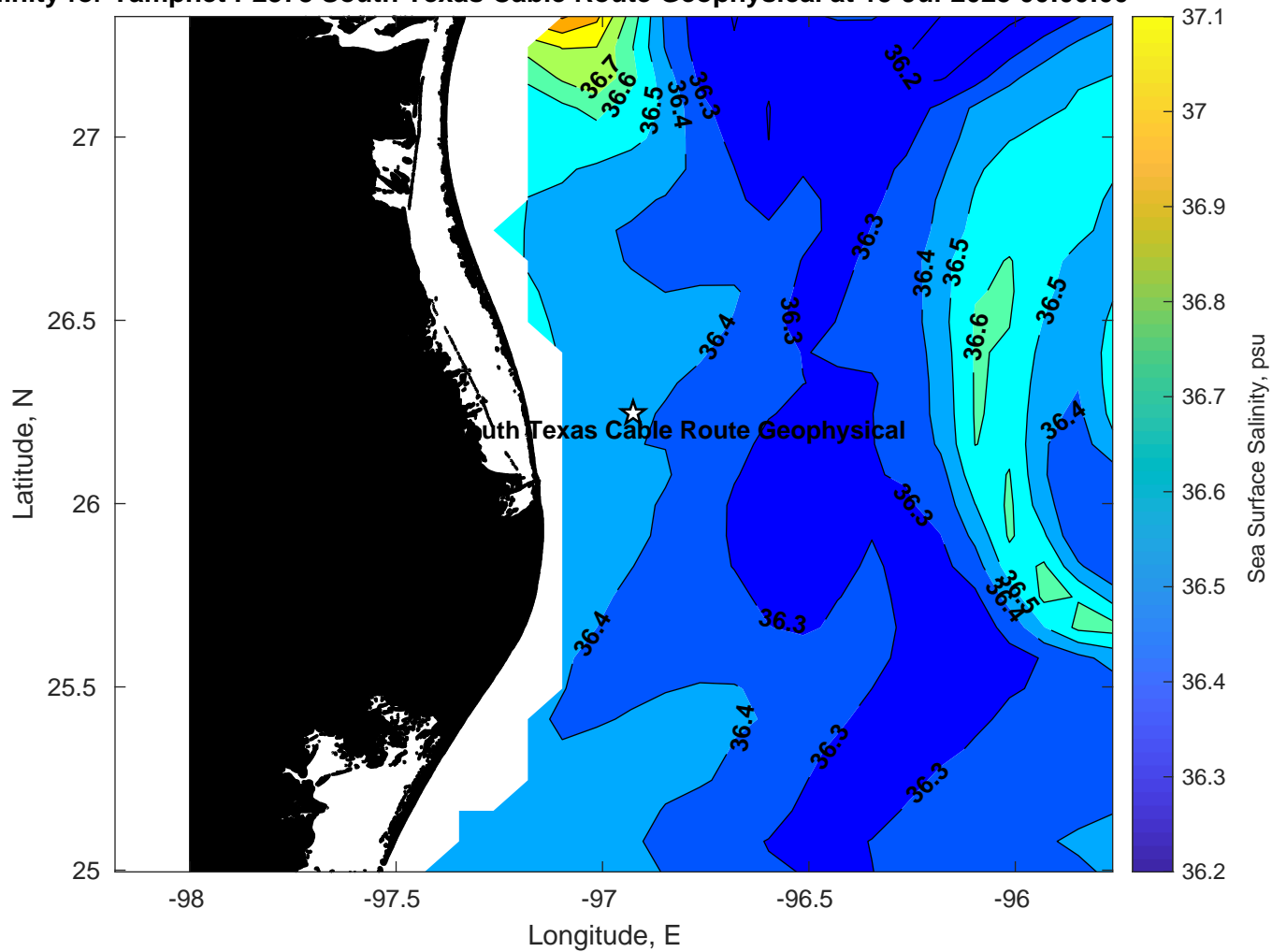
Surface Salinity for Tampnet P2378 South Texas Cable Route Geophysical at 15-Jul-2025 00:00:00
