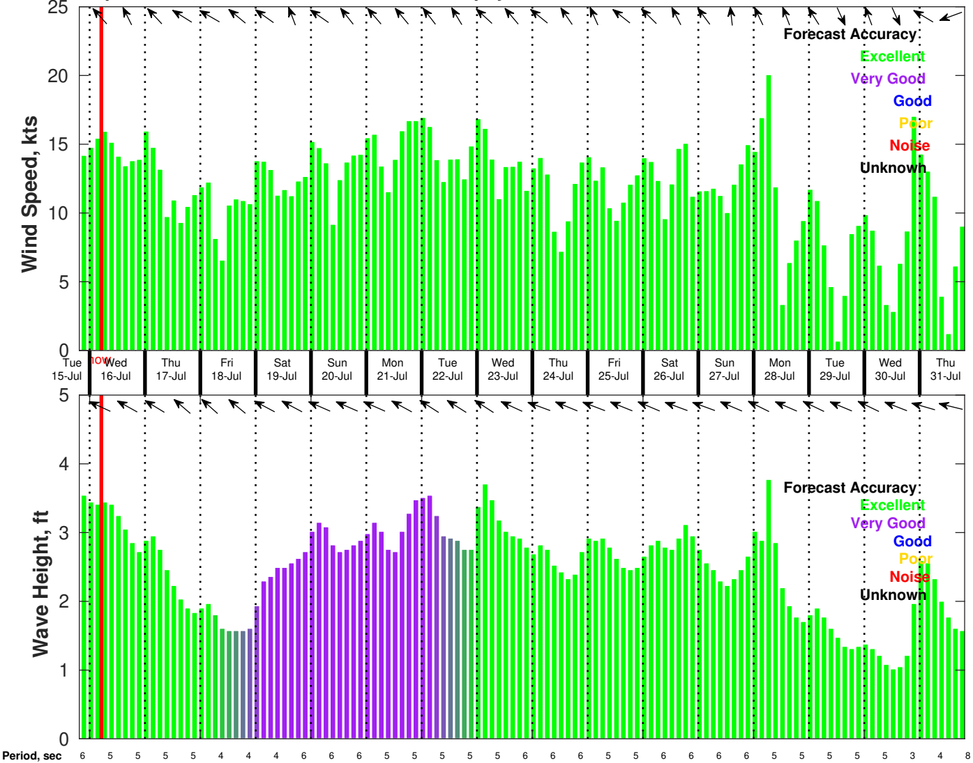
Wind & Wave Forecast for Tampnet P2378 South Texas Cable Route Geophysical from 15-Jul-2025 20:00:00 to 31-Jul-2025 20:00:00
