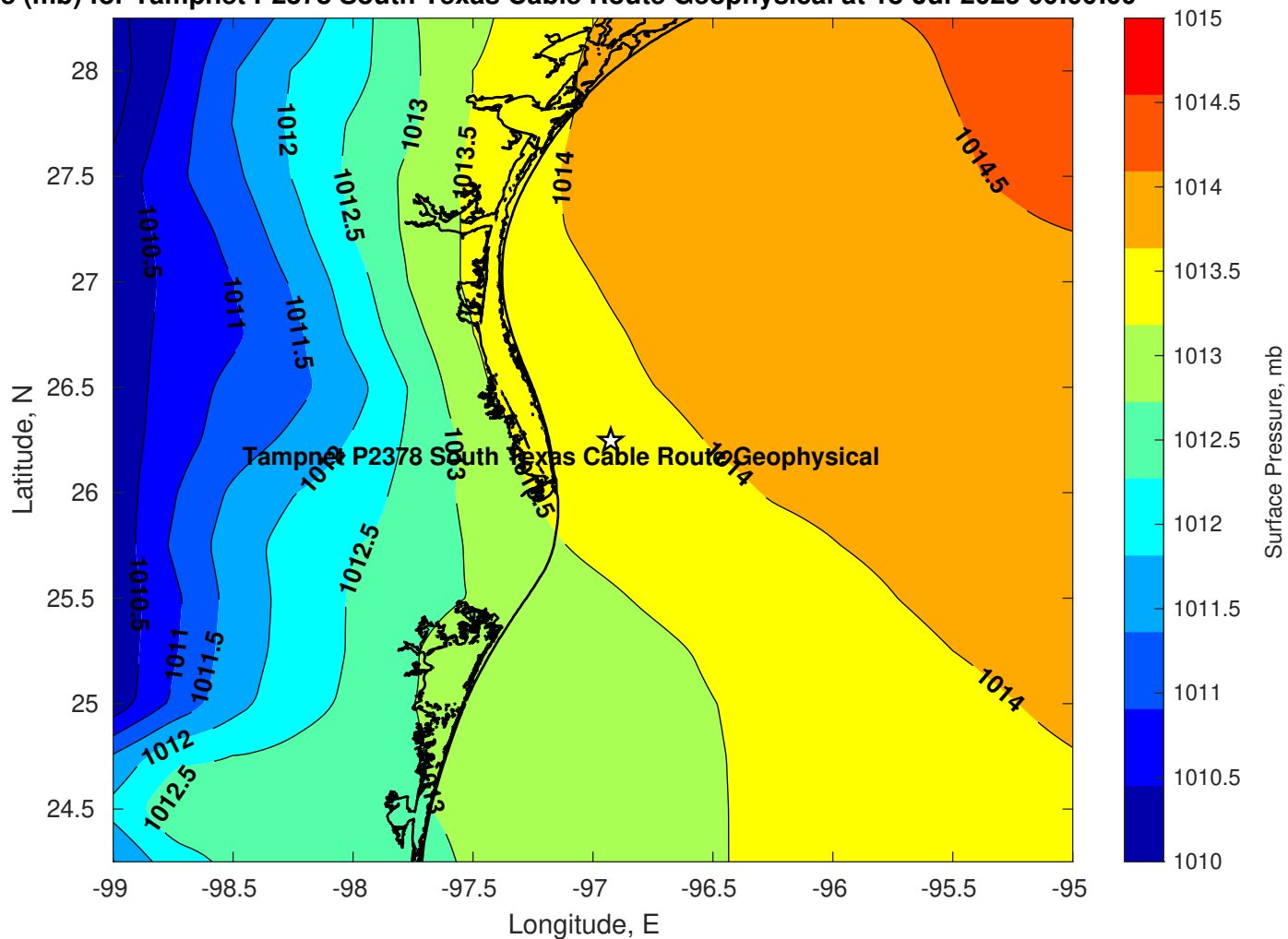
Pressure (mb) for Tampnet P2378 South Texas Cable Route Geophysical at 18-Jul-2025 00:00:00
