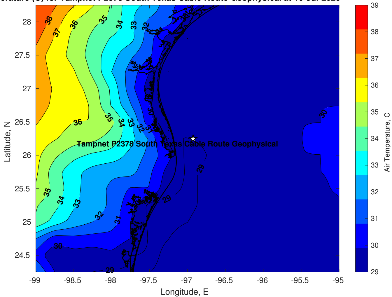
Air Temperature (C) for Tampnet P2378 South Texas Cable Route Geophysical at 16-Jul-2025
