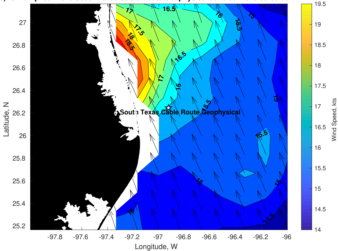
Winds (kts) for Tampnet P2378 South Texas Cable Route Geophysical at 16-Jul-2025 09:00:00
