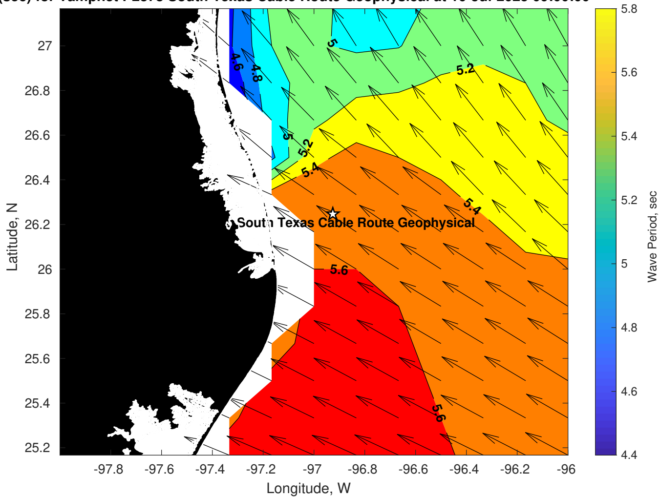
Wave Period (sec) for Tampnet P2378 South Texas Cable Route Geophysical at 16-Jul-2025 09:00:00
