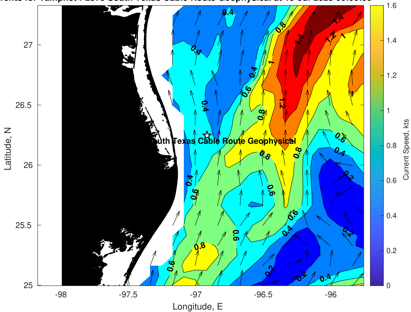
Surface Currents for Tampnet P2378 South Texas Cable Route Geophysical at 15-Jul-2025 00:00:00
