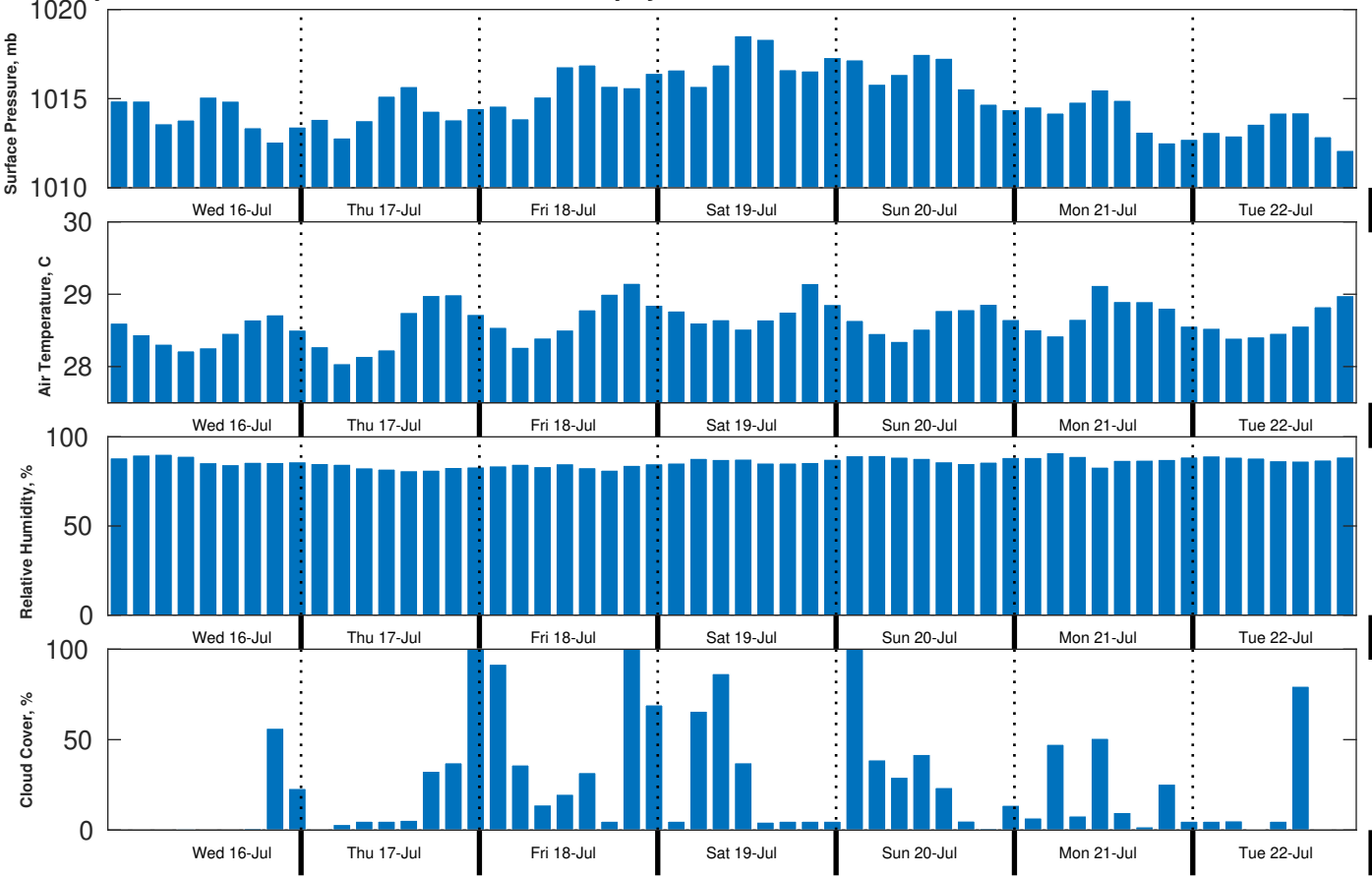
Met Forecast for Tampnet P2378 South Texas Cable Route Geophysical from 16-Jul-2025 00:00:00 to 23-Jul-2025 00:00:00
