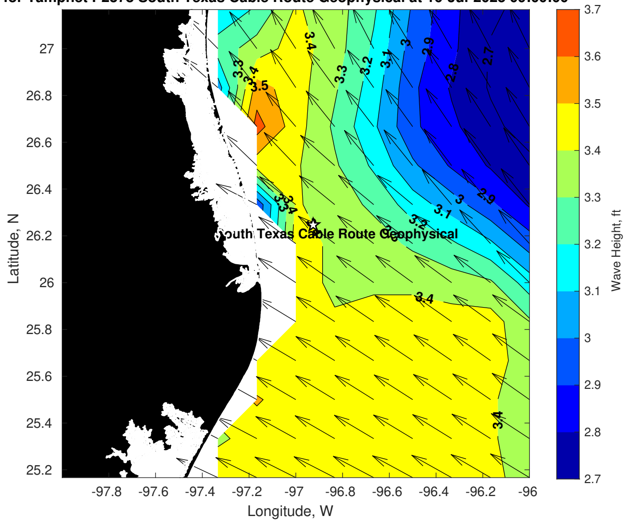
Wave Height (ft) for Tampnet P2378 South Texas Cable Route Geophysical at 16-Jul-2025 09:00:00
