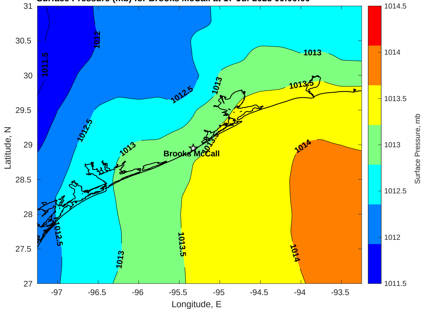
Surface Pressure (mb) for Brooks McCall at 17-Jul-2025 00:00:00
