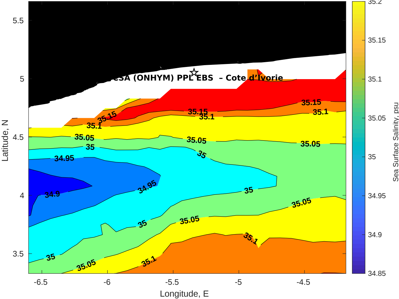
Surface Salinity for CSA (ONHYM) PPL EBS - Cote d'Ivoire at 16-Jul-2025 00:00:00
