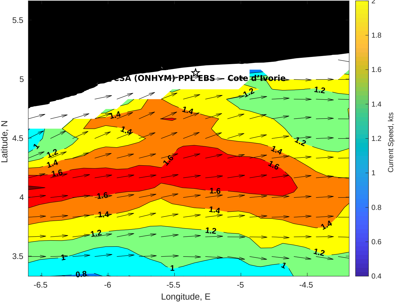
Surface Currents for CSA (ONHYM) PPL EBS - Cote d'Ivoire at 16-Jul-2025 00:00:00
