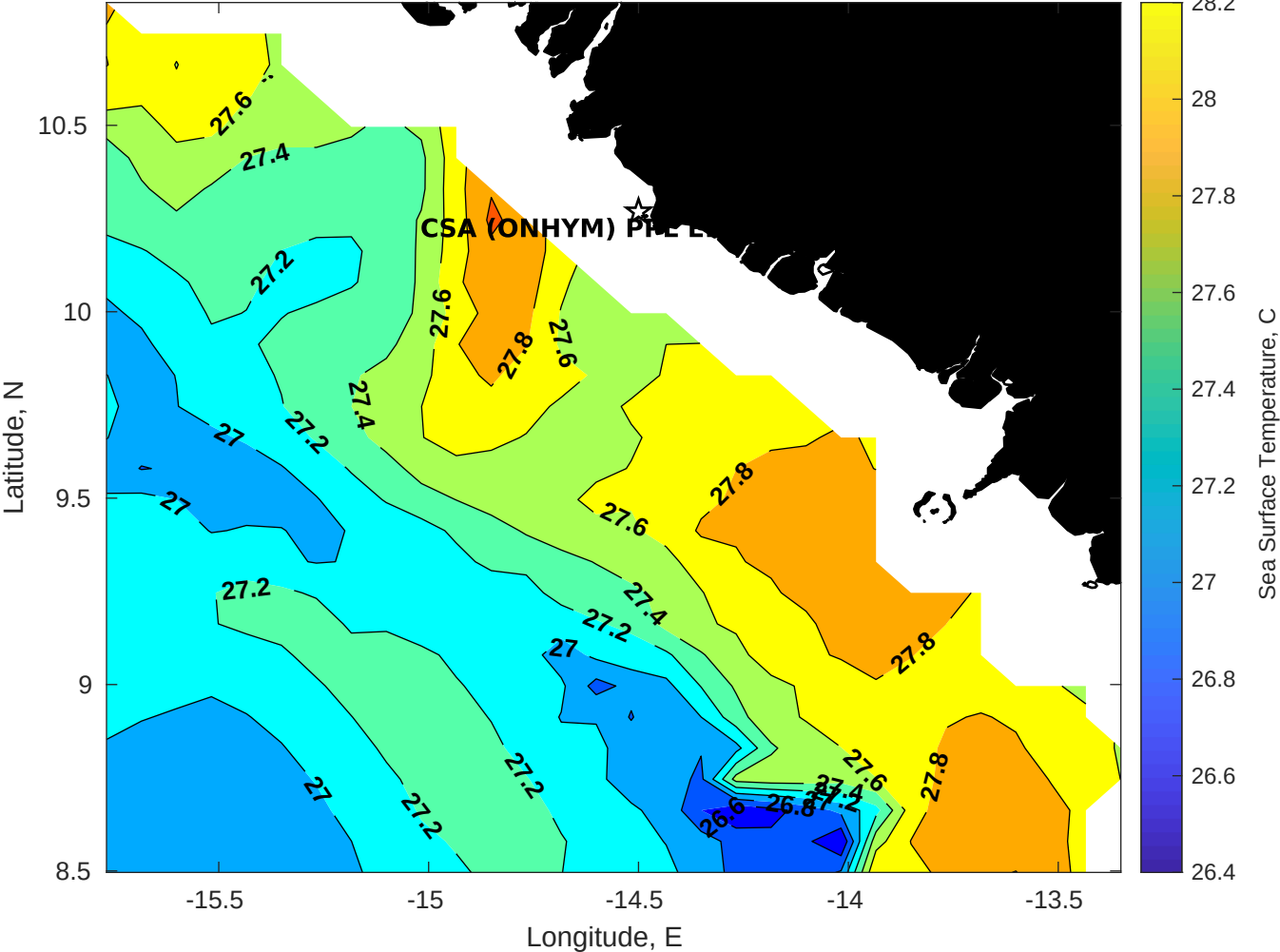
SST for CSA (ONHYM) PPL EBS - Guinea at 16-Jul-2025 00:00:00
