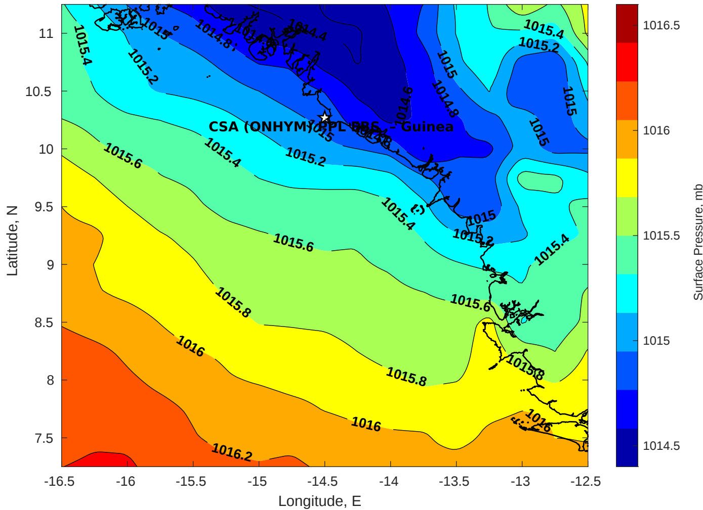
Surface Pressure (mb) for CSA (ONHYM) PPL EBS - Guinea at 17-Jul-2025 12:00:00
