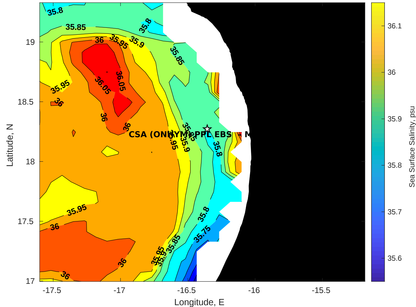
Surface Salinity for CSA (ONHYM) PPL EBS - Mauritania at 16-Jul-2025 00:00:00
