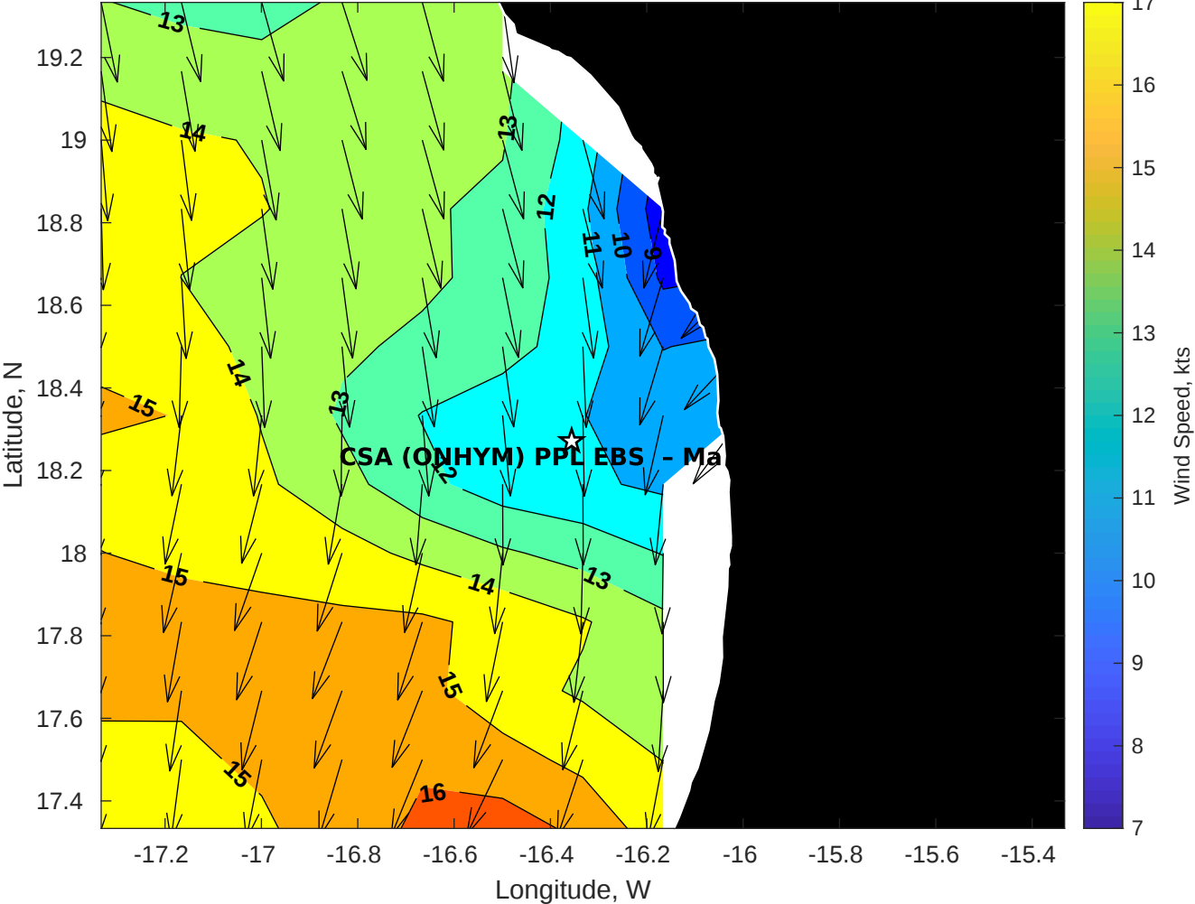
Winds (kts) for CSA (ONHYM) PPL EBS - Mauritania at 17-Jul-2025 09:00:00
