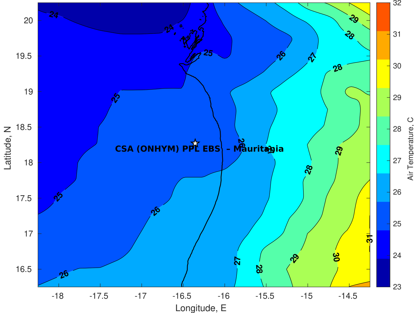
Air Temperature (C) for CSA (ONHYM) PPL EBS - Mauritania at 17-Jul-2025
