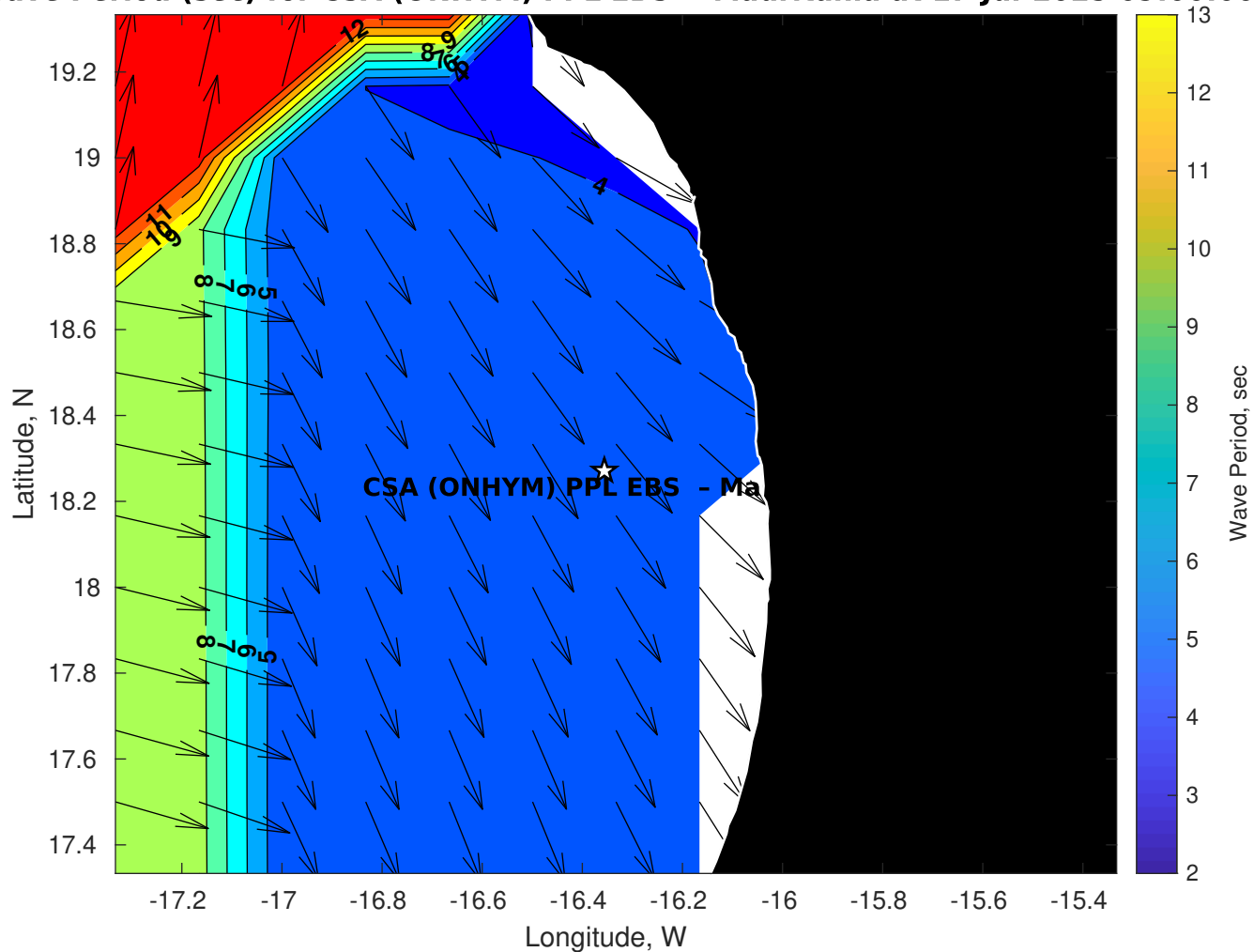
Wave Period (sec) for CSA (ONHYM) PPL EBS - Mauritania at 17-Jul-2025 09:00:00
