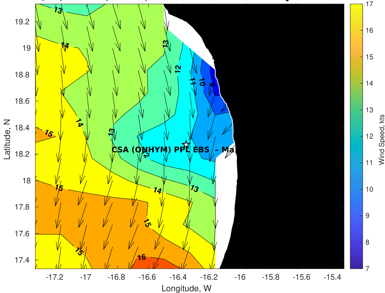
Winds (kts) for CSA (ONHYM) PPL EBS - Mauritania at 17-Jul-2025 09:00:00
