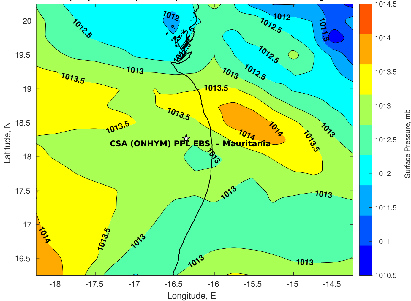
Surface Pressure (mb) for CSA (ONHYM) PPL EBS - Mauritania at 19-Jul-2025 00:00:00
