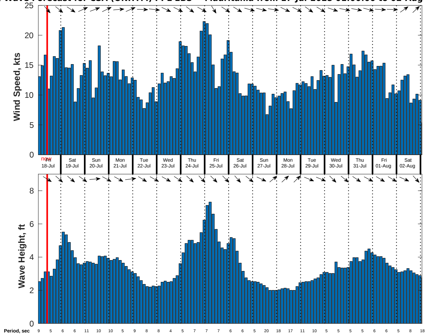
Wind & Wave Forecast for CSA (ONHYM) PPL EBS - Mauritania from 17-Jul-2025 01:00:00 to 02-Aug-2025 01:00:00
