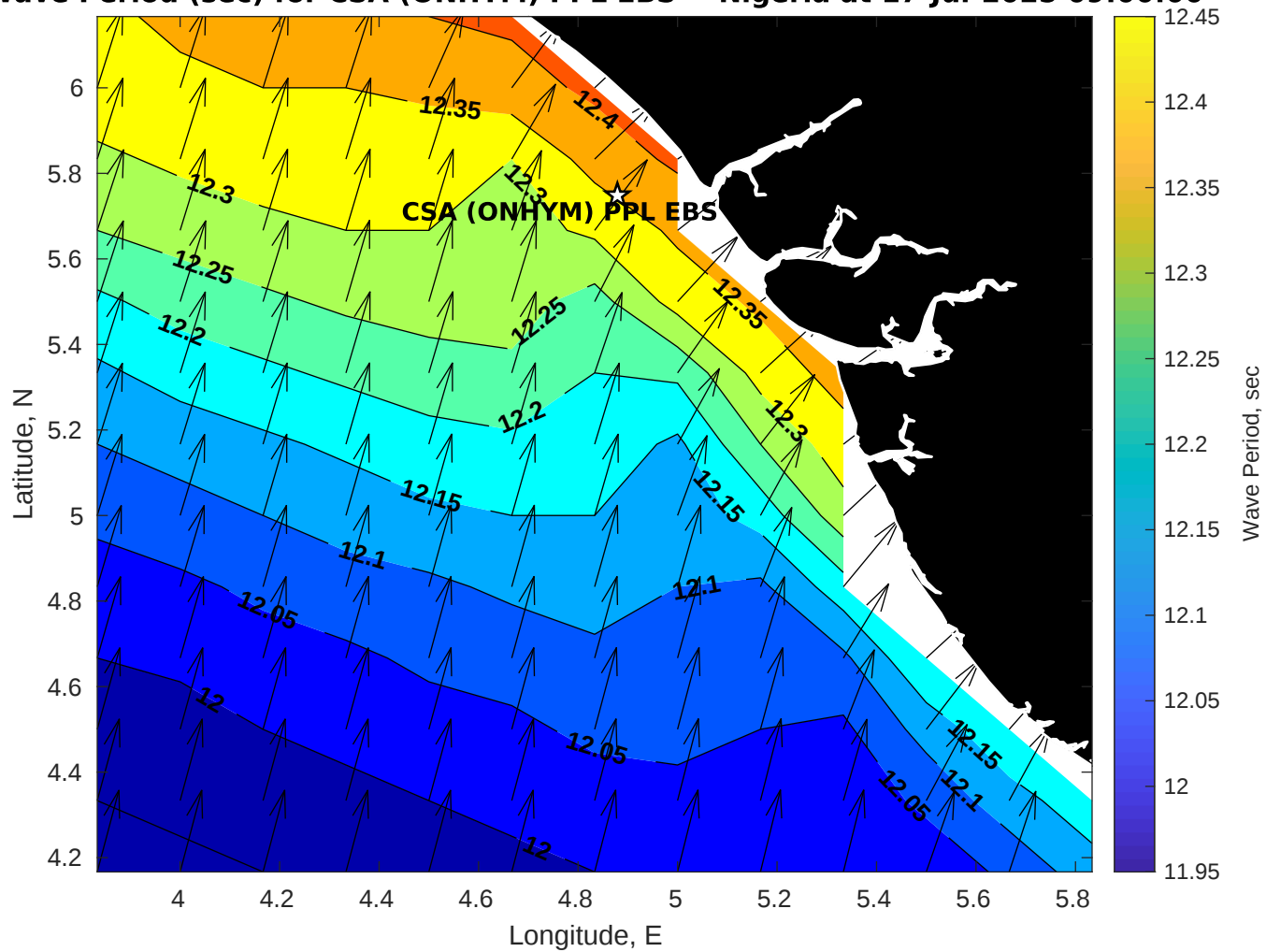
Wave Period (sec) for CSA (ONHYM) PPL EBS - Nigeria at 17-Jul-2025 09:00:00
