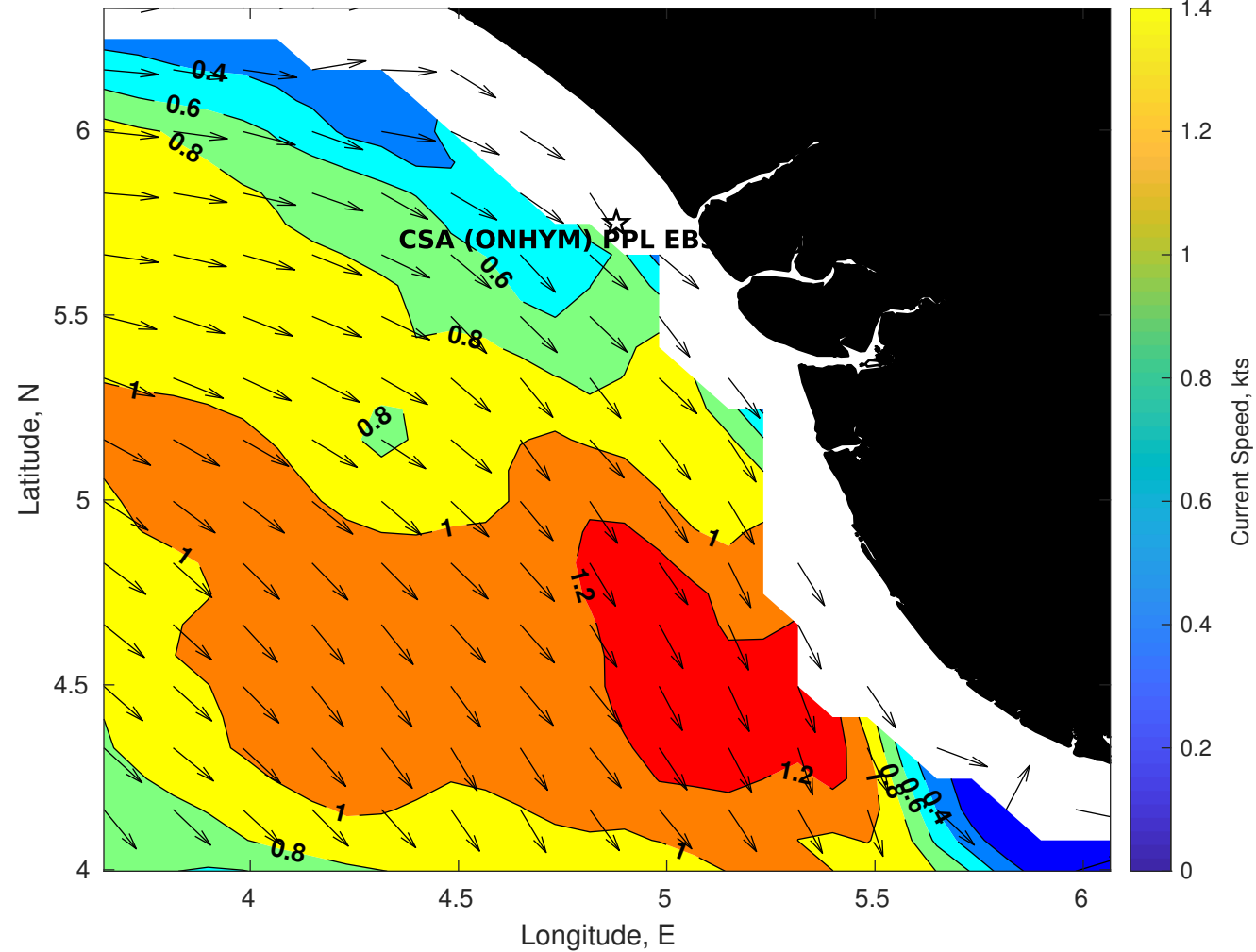
Surface Currents for CSA (ONHYM) PPL EBS - Nigeria at 16-Jul-2025 00:00:00
