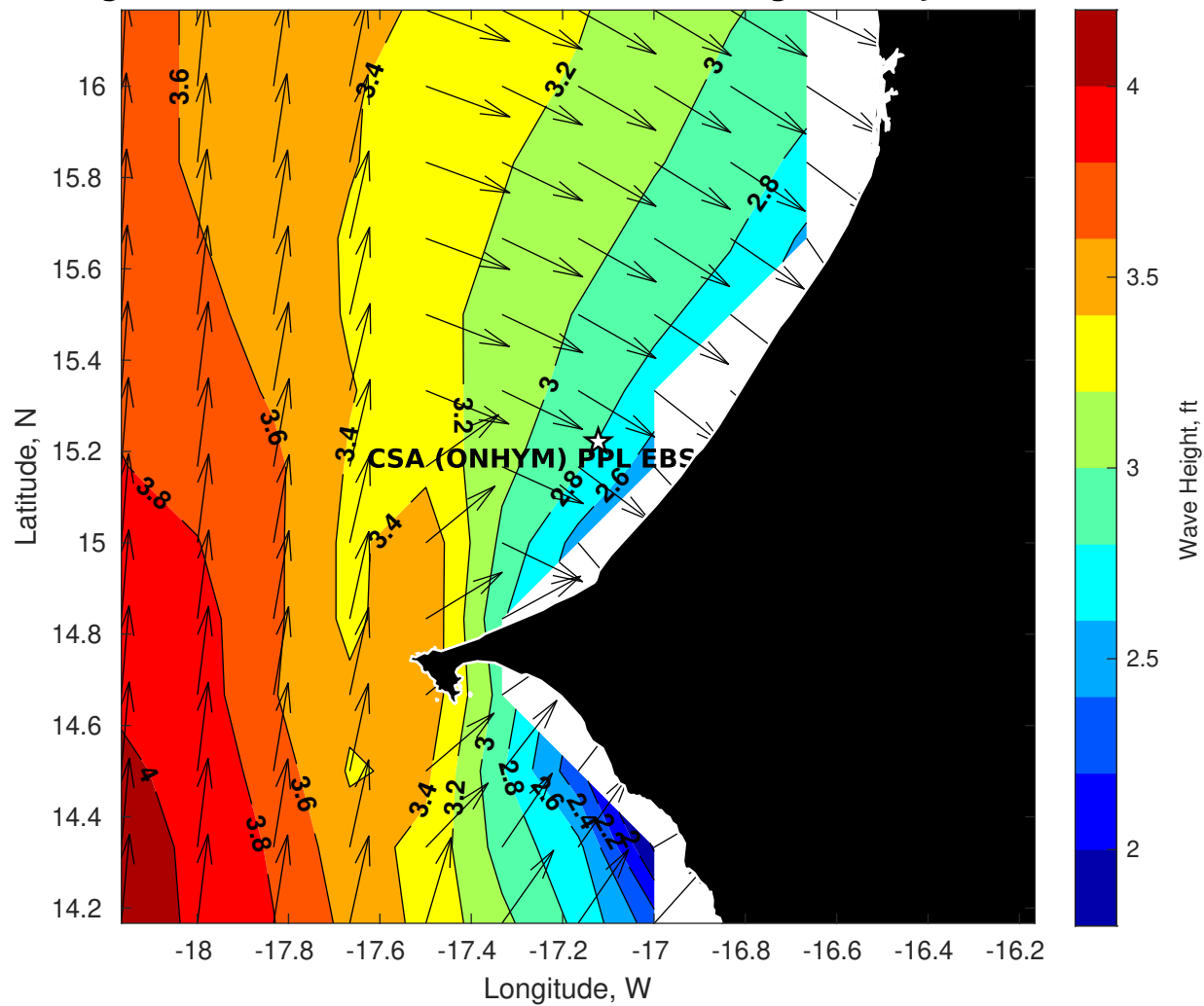
Wave Height (ft) for CSA (ONHYM) PPL EBS - Senegal at 17-Jul-2025 09:00:00
