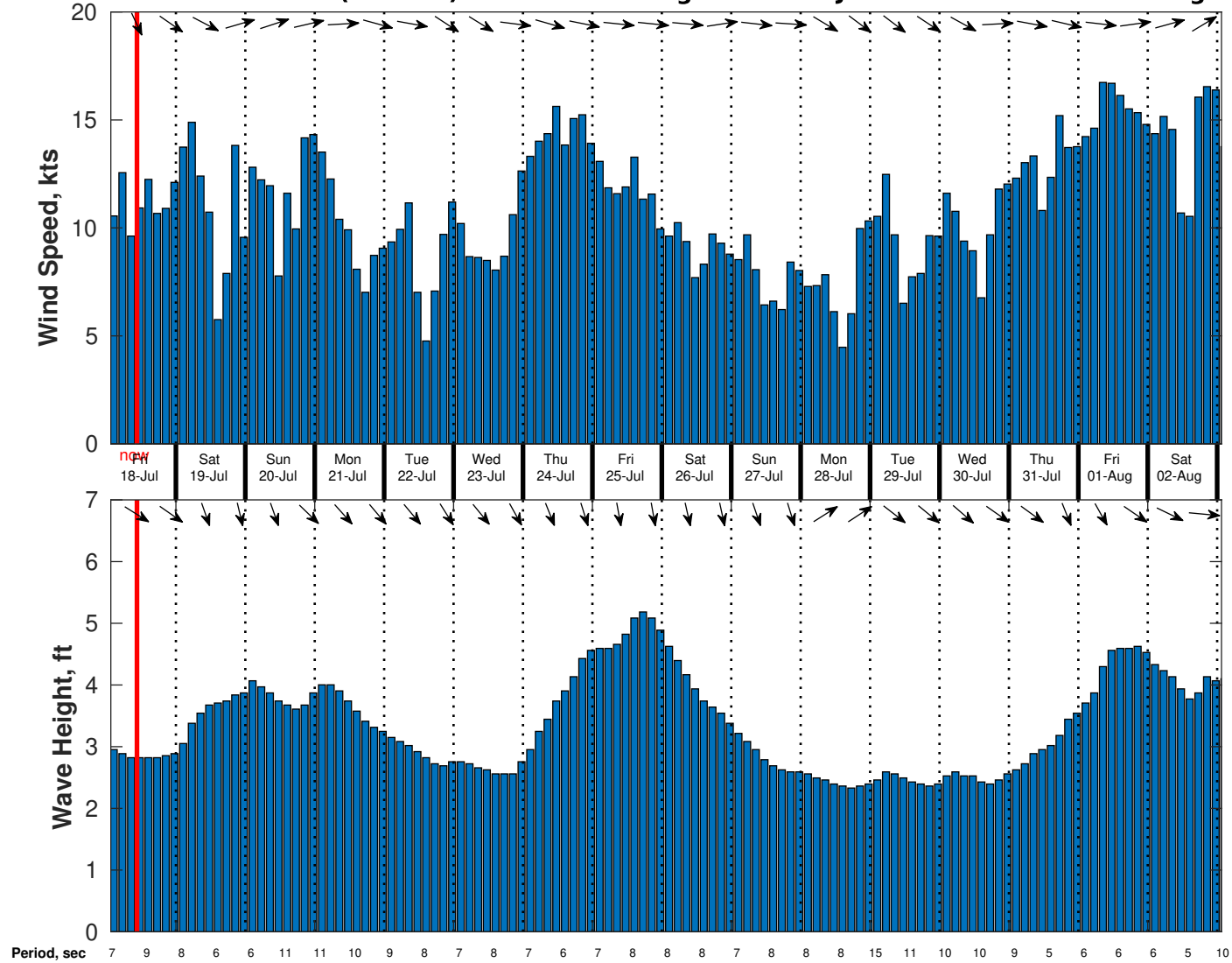
Wind & Wave Forecast for CSA (ONHYM) PPL EBS - Senegal from 17-Jul-2025 01:00:00 to 02-Aug-2025 01:00:00
