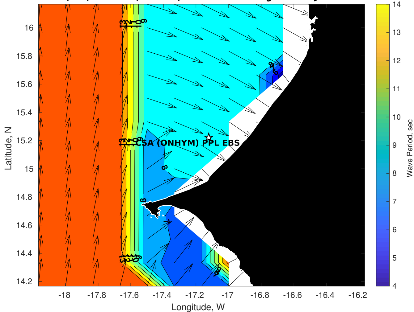
Wave Period (sec) for CSA (ONHYM) PPL EBS - Senegal at 17-Jul-2025 09:00:00
