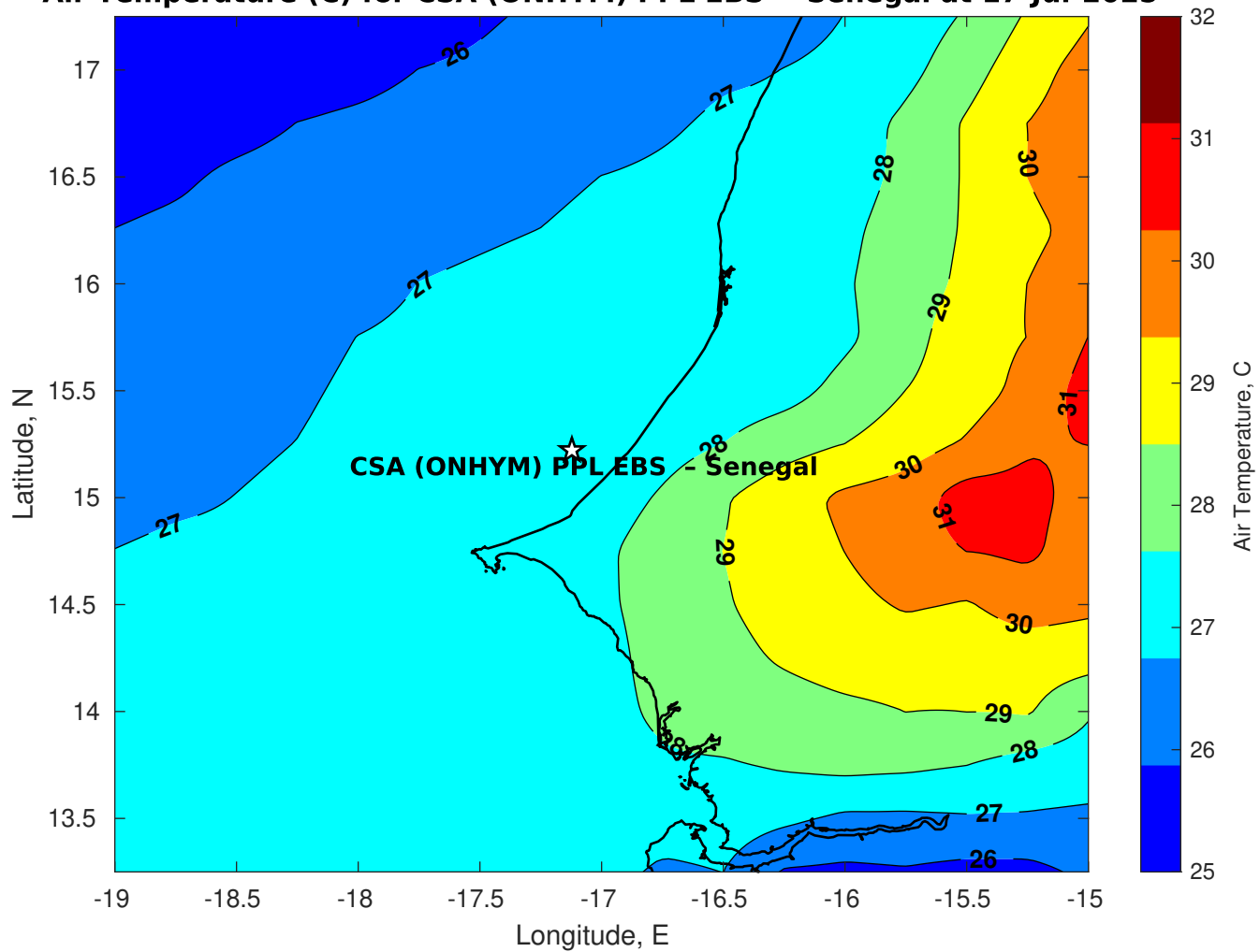
Air Temperature (C) for CSA (ONHYM) PPL EBS - Senegal at 17-Jul-2025
