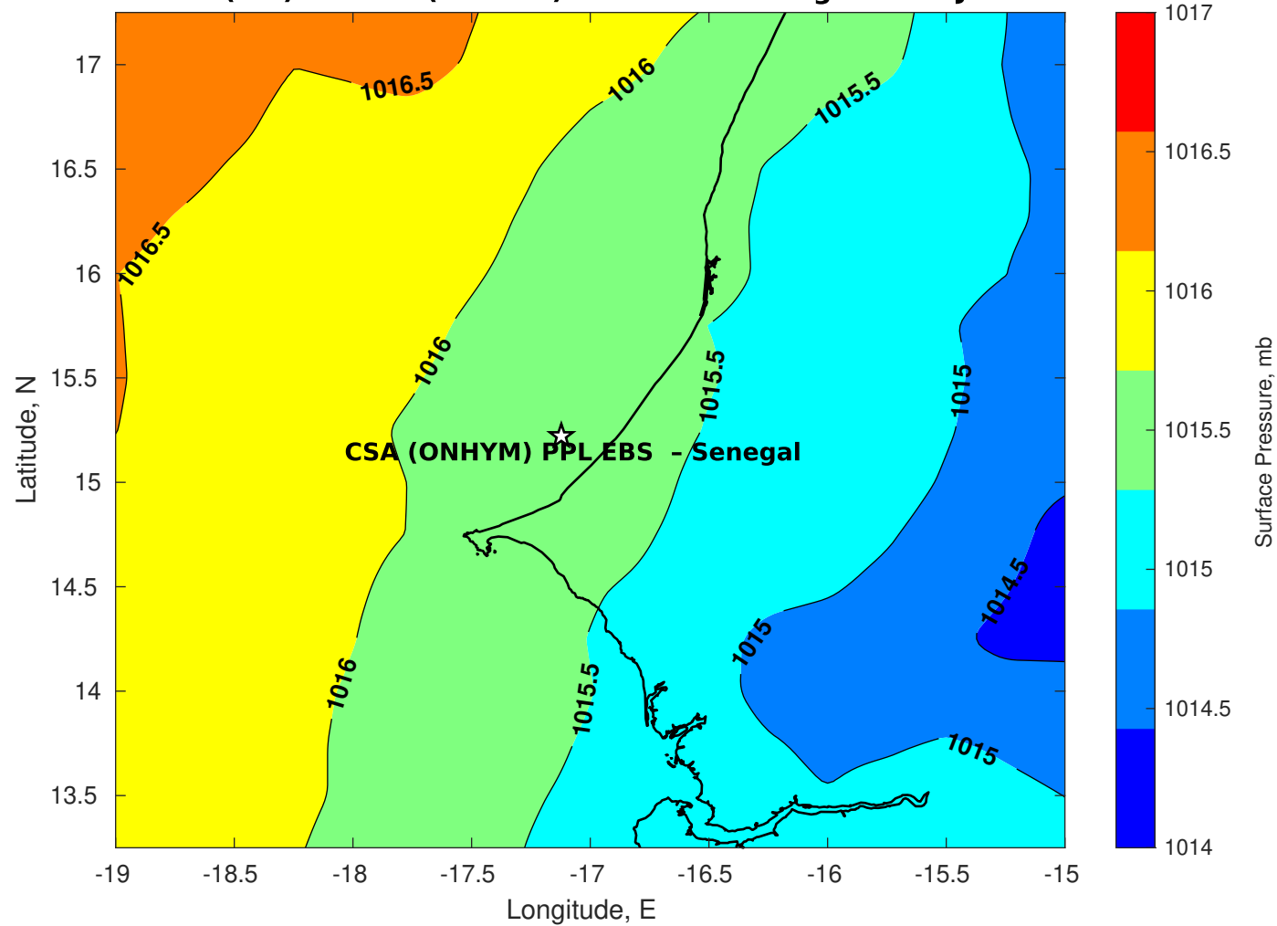
Surface Pressure (mb) for CSA (ONHYM) PPL EBS - Senegal at 17-Jul-2025 00:00:00
