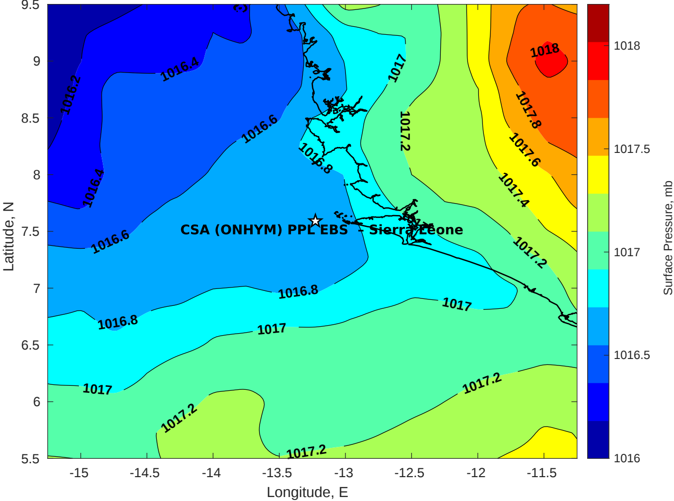
Surface Pressure (mb) for CSA (ONHYM) PPL EBS - Sierra Leone at 19-Jul-2025 00:00:00
