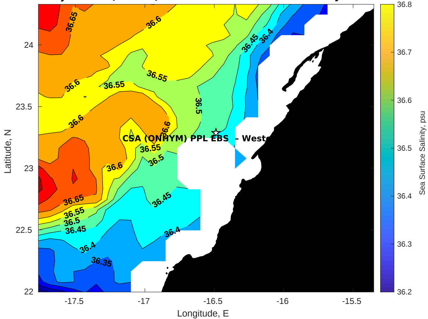
Surface Salinity for CSA (ONHYM) PPL EBS - Western Sahara at 16-Jul-2025 00:00:00
