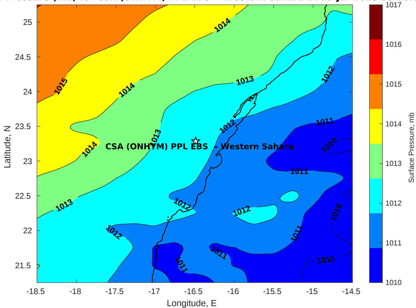
Surface Pressure (mb) for CSA (ONHYM) PPL EBS - Western Sahara at 19-Jul-2025 00:00:00
