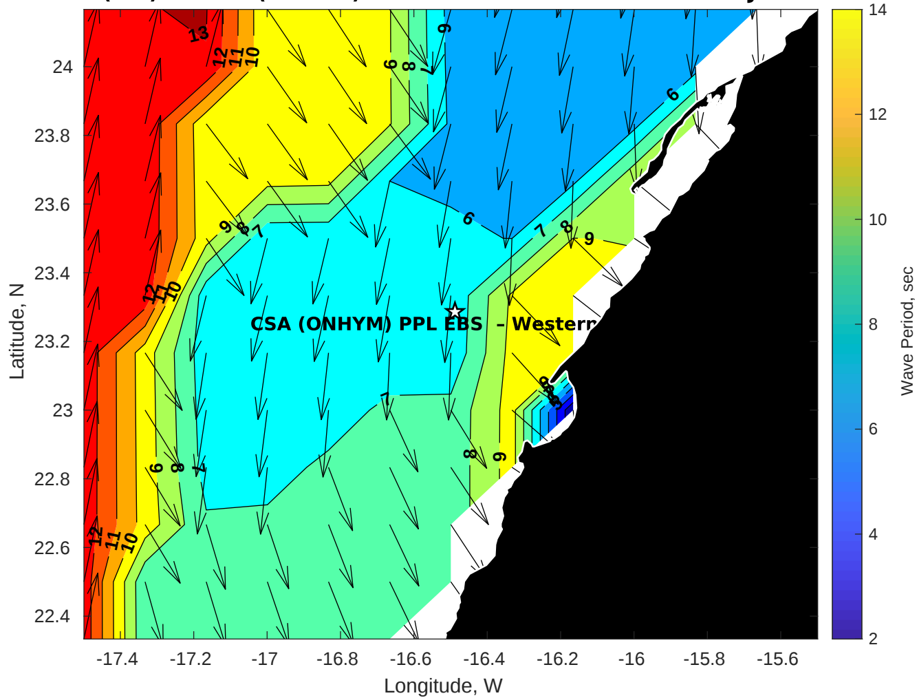
Wave Period (sec) for CSA (ONHYM) PPL EBS - Western Sahara at 17-Jul-2025 09:00:00
