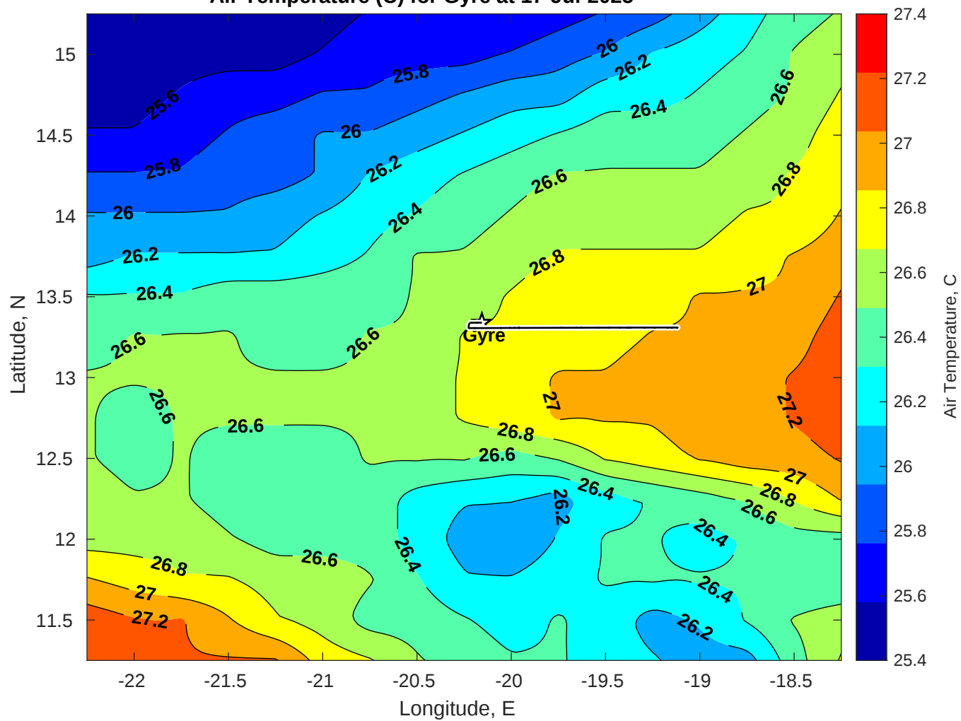
Air Temperature (C) for Gyre at 17-Jul-2025
