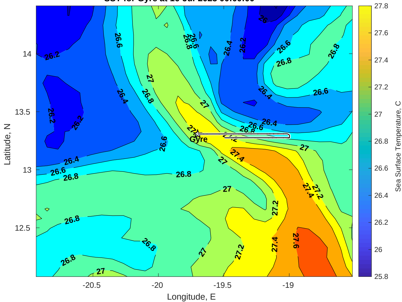
SST for Gyre at 16-Jul-2025 00:00:00
