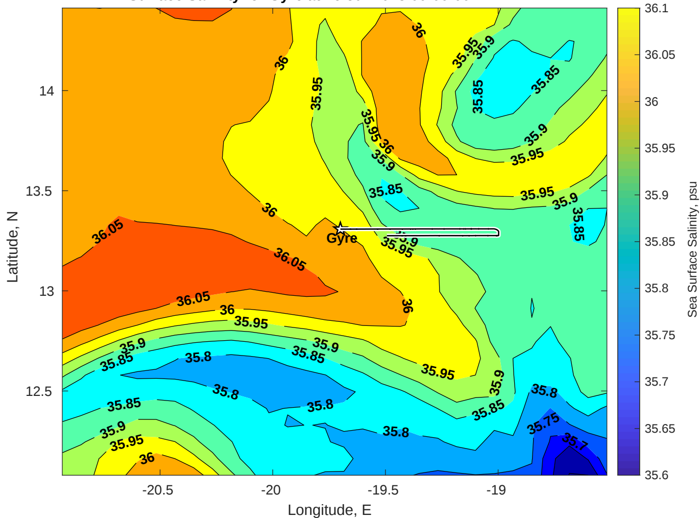
Surface Salinity for Gyre at 16-Jul-2025 00:00:00
