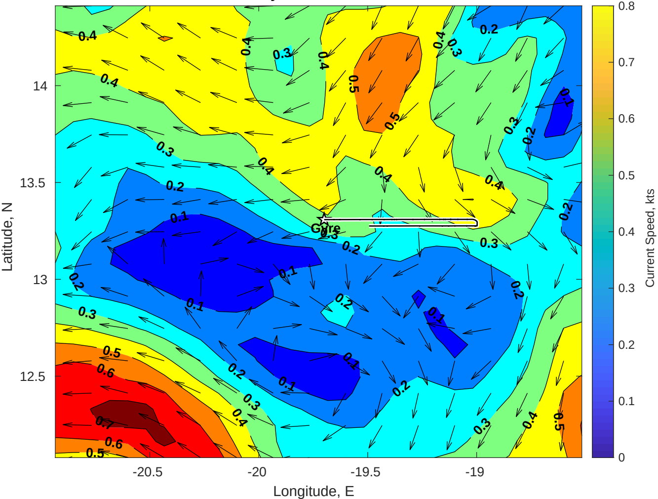
Surface Currents for Gyre at 16-Jul-2025 00:00:00
