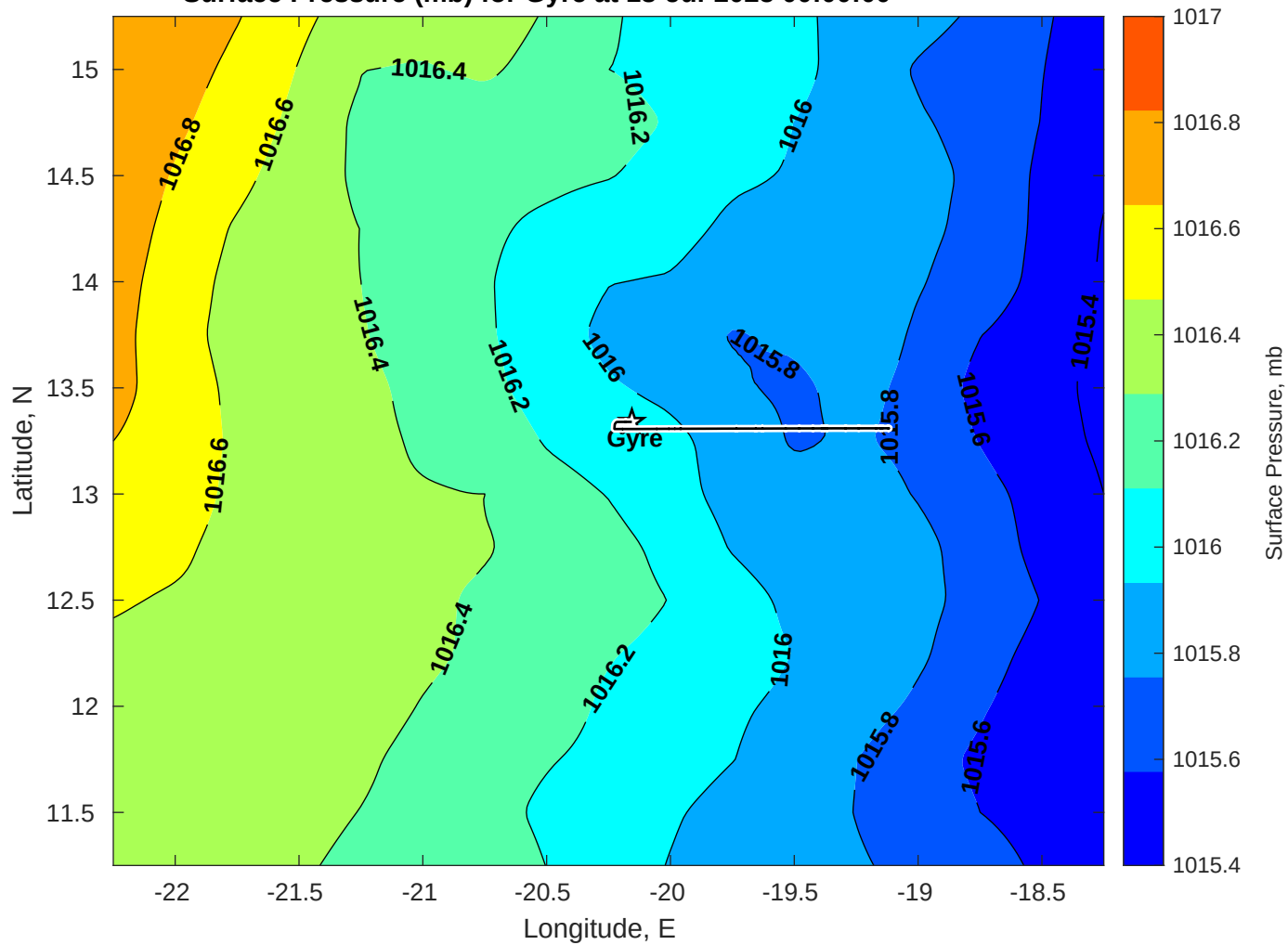
Surface Pressure (mb) for Gyre at 18-Jul-2025 00:00:00
