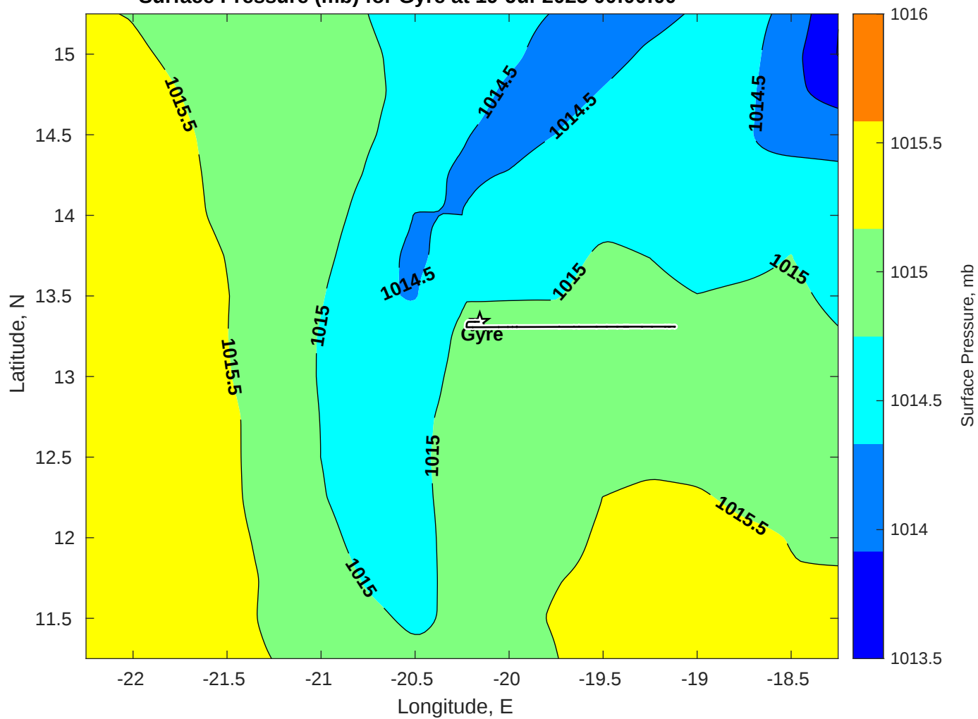
Surface Pressure (mb) for Gyre at 19-Jul-2025 00:00:00
