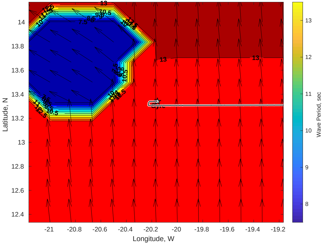
Wave Period (sec) for Gyre at 17-Jul-2025 09:00:00
