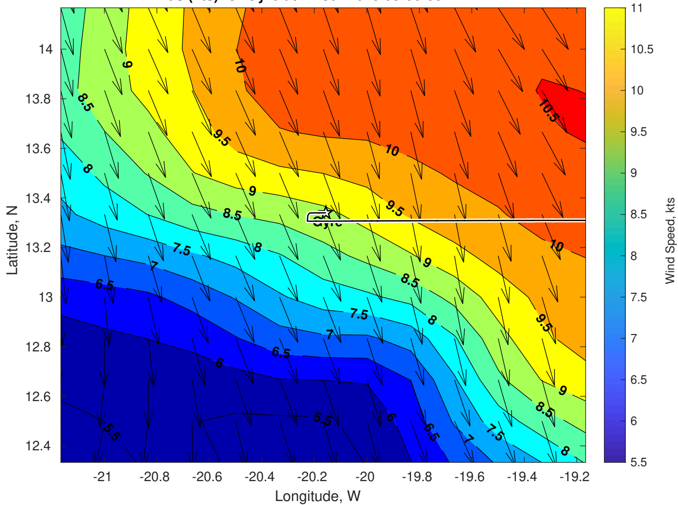
Winds (kts) for Gyre at 17-Jul-2025 09:00:00
