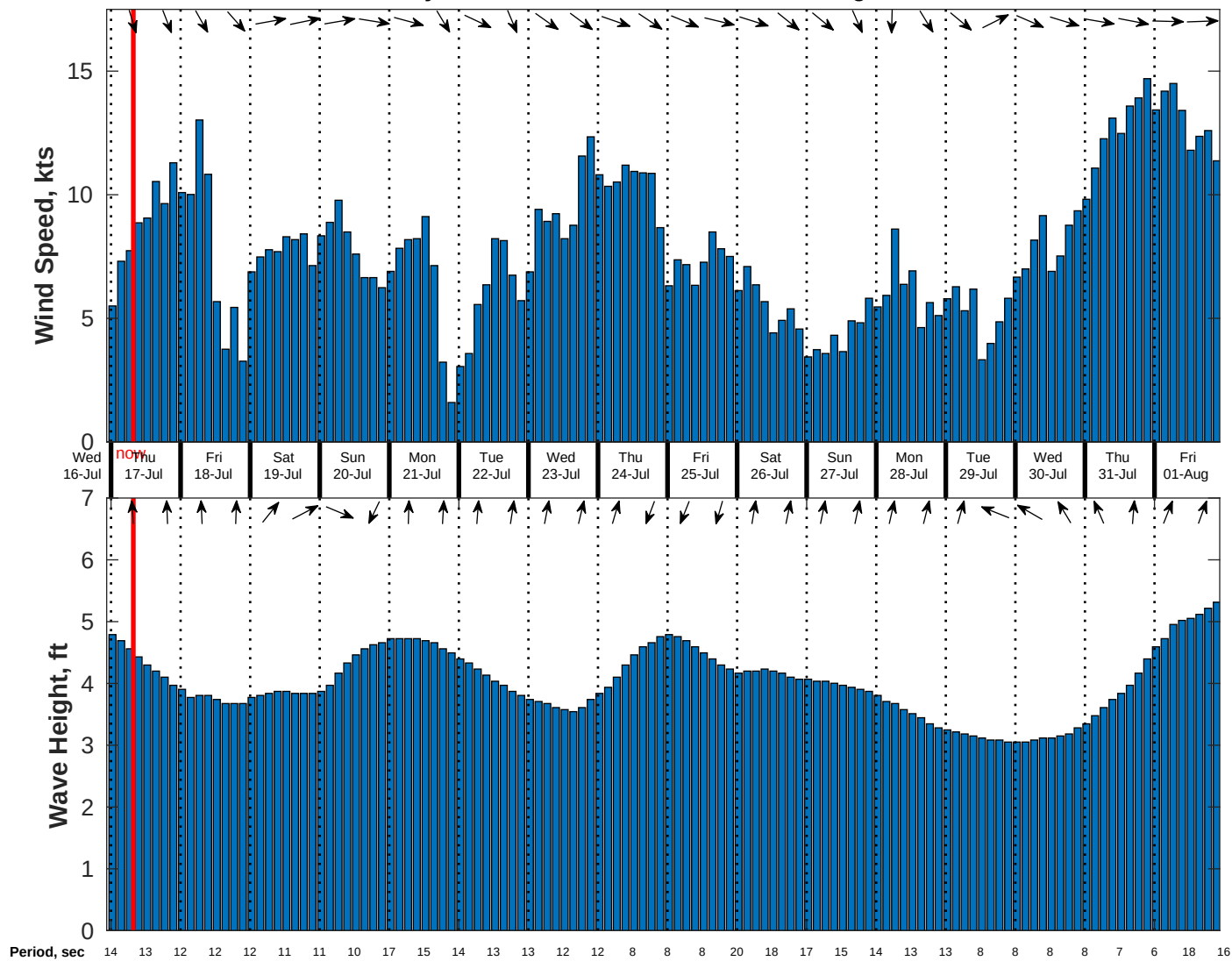
Wind & Wave Forecast for Gyre from 16-Jul-2025 23:00:00 to 01-Aug-2025 23:00:00
