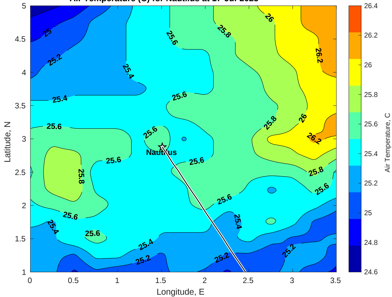
Air Temperature (C) for Nautilus at 17-Jul-2025
