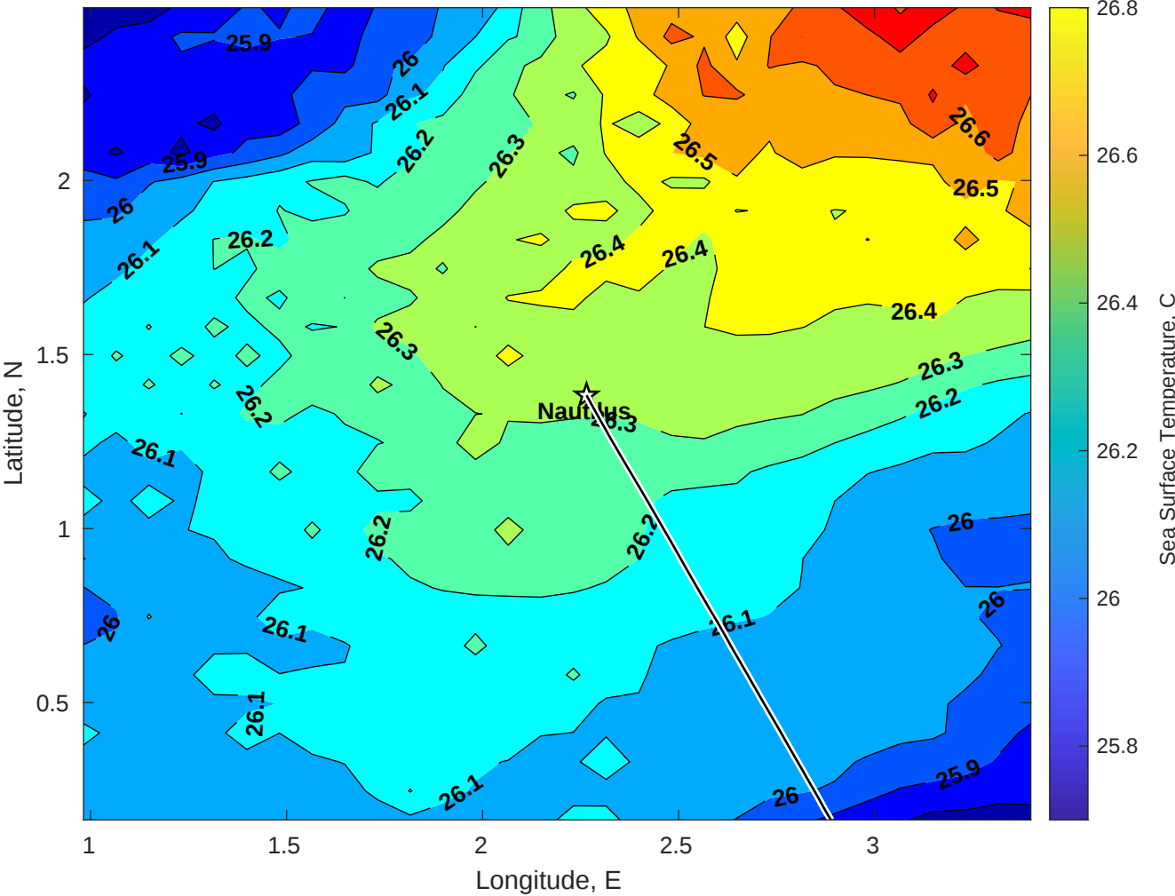
SST for Nautilus at 16-Jul-2025 00:00:00
