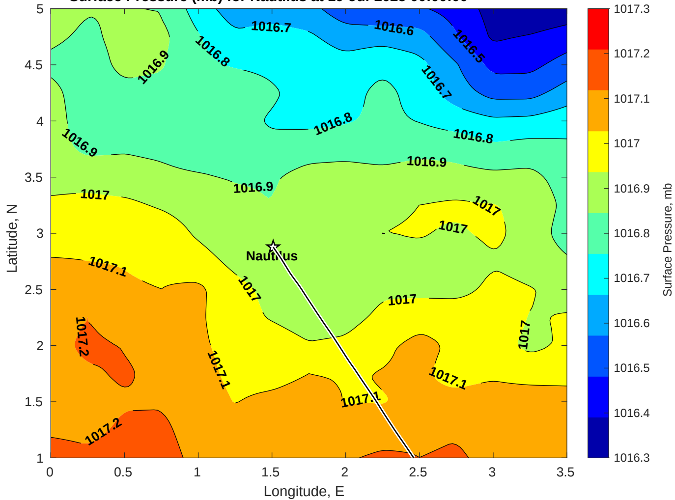
Surface Pressure (mb) for Nautilus at 19-Jul-2025 00:00:00
