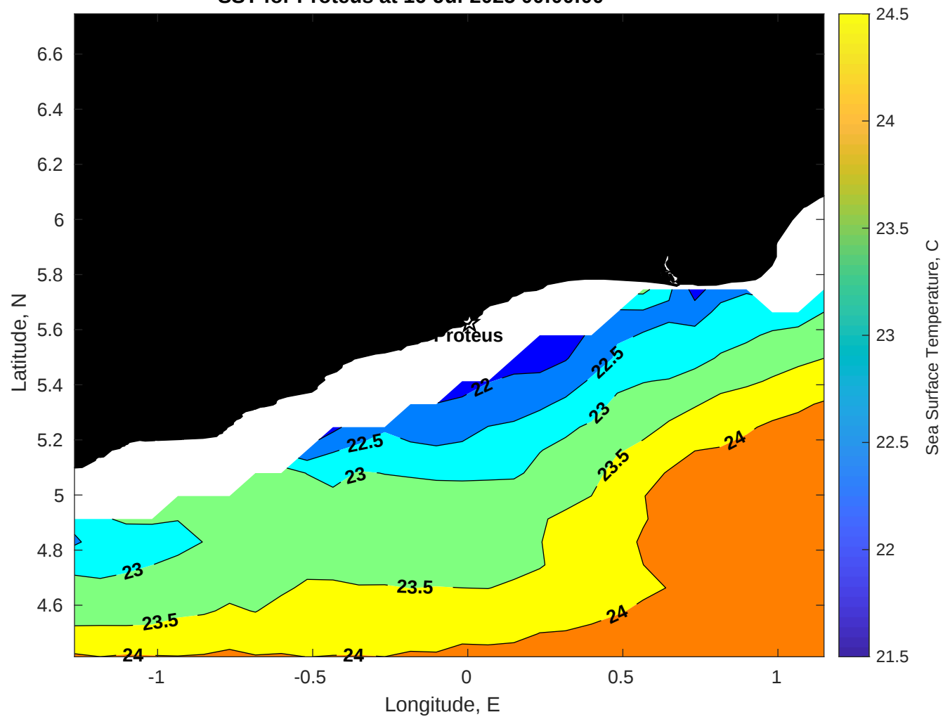
SST for Proteus at 16-Jul-2025 00:00:00
