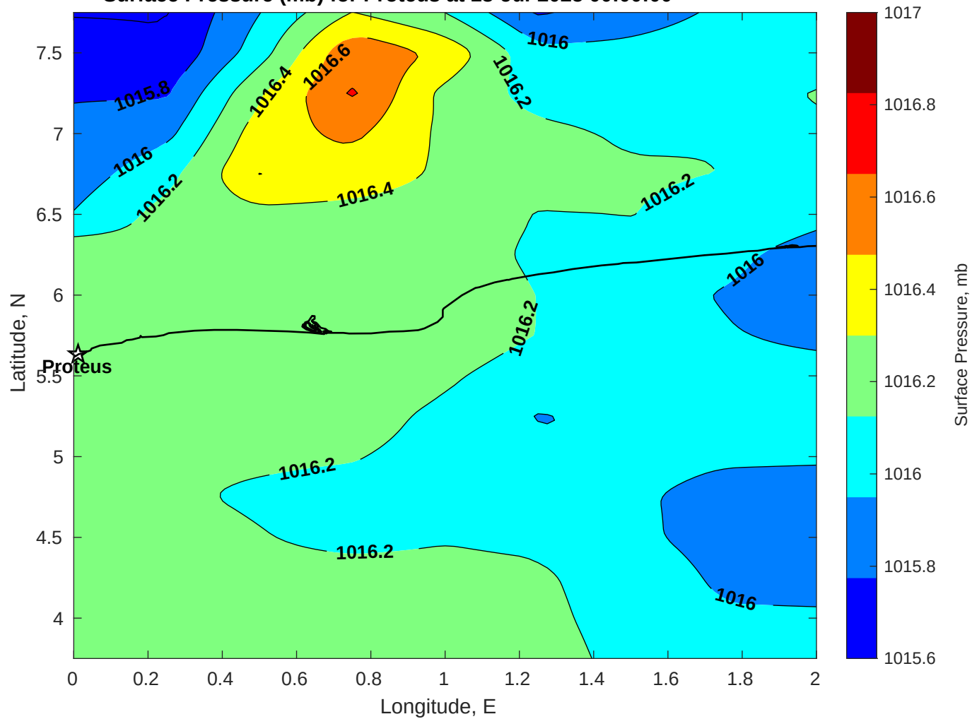
Surface Pressure (mb) for Proteus at 18-Jul-2025 00:00:00
