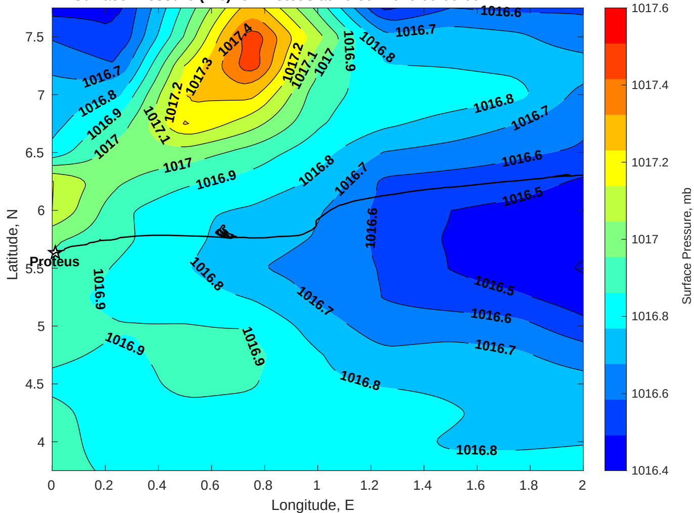
Surface Pressure (mb) for Proteus at 19-Jul-2025 00:00:00
