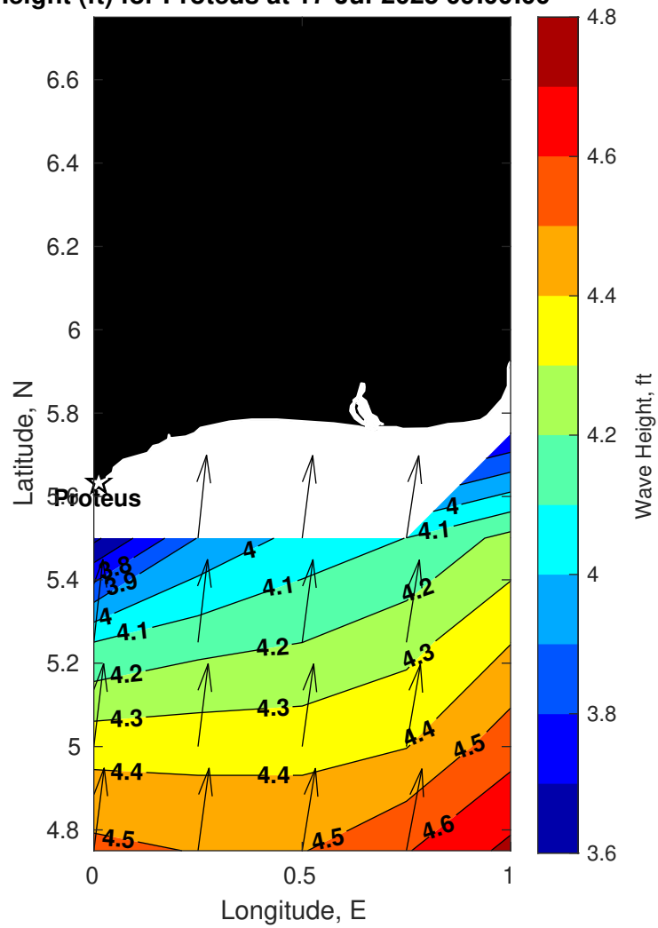
Wave Height (ft) for Proteus at 17-Jul-2025 09:00:00
