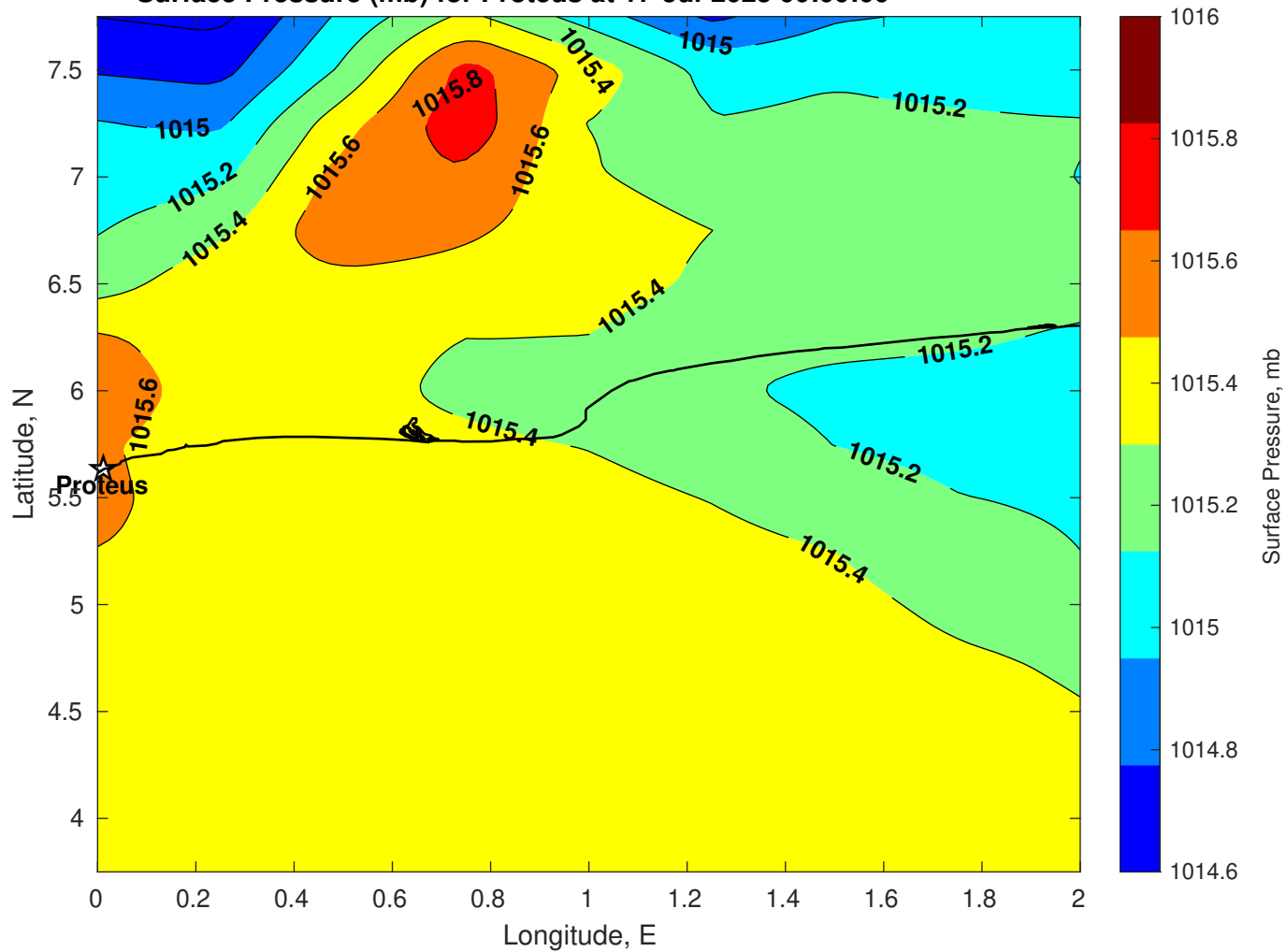
Surface Pressure (mb) for Proteus at 17-Jul-2025 00:00:00
