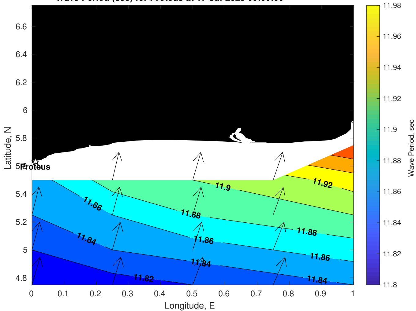
Wave Period (sec) for Proteus at 17-Jul-2025 09:00:00
