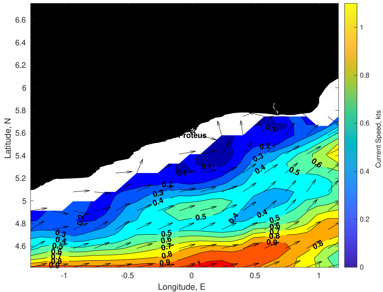
Surface Currents for Proteus at 16-Jul-2025 00:00:00
