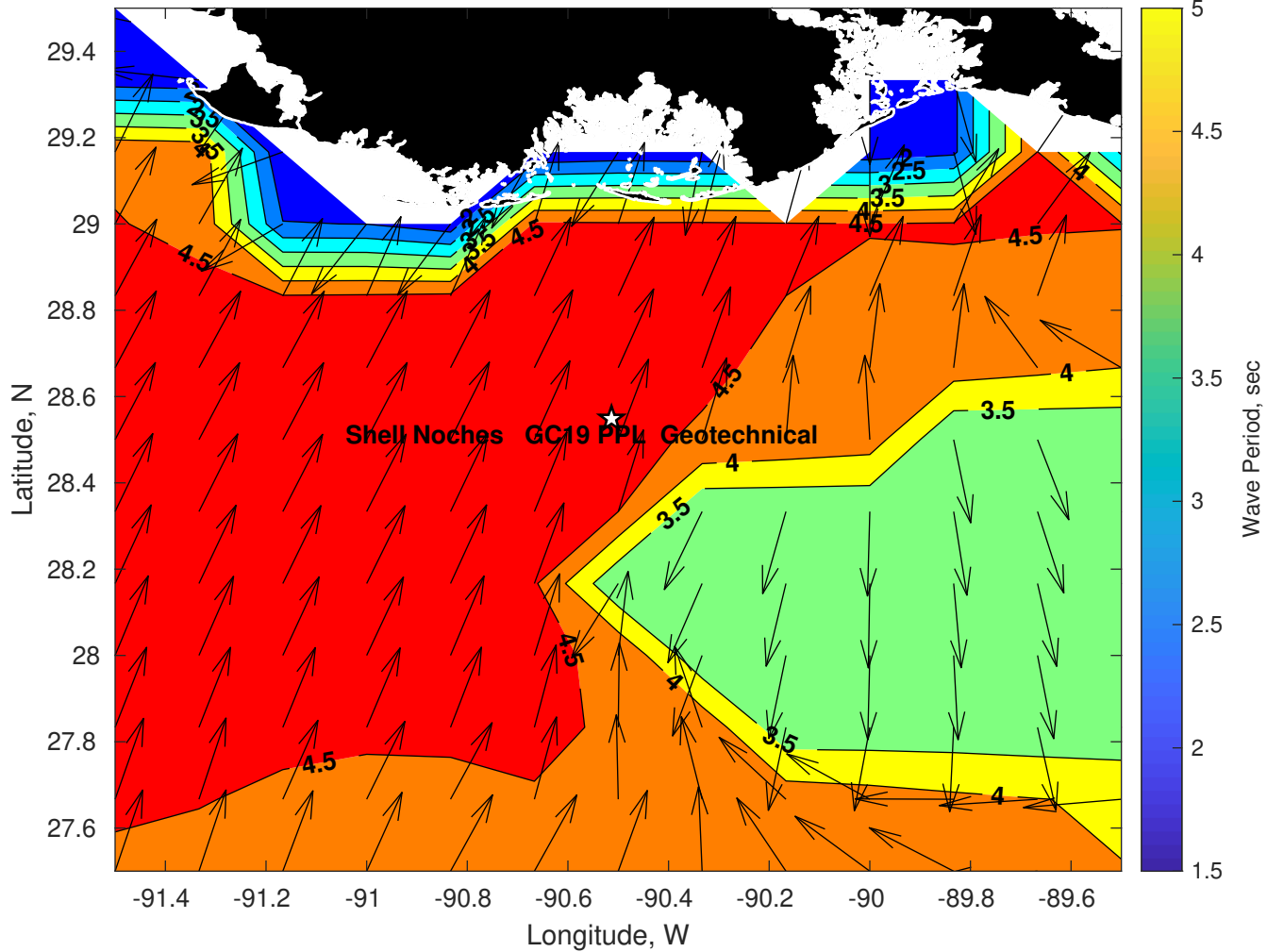
Wave Period (sec) for Shell Noches GC19 PPL Geotechnical at 17-Jul-2025 09:00:00
