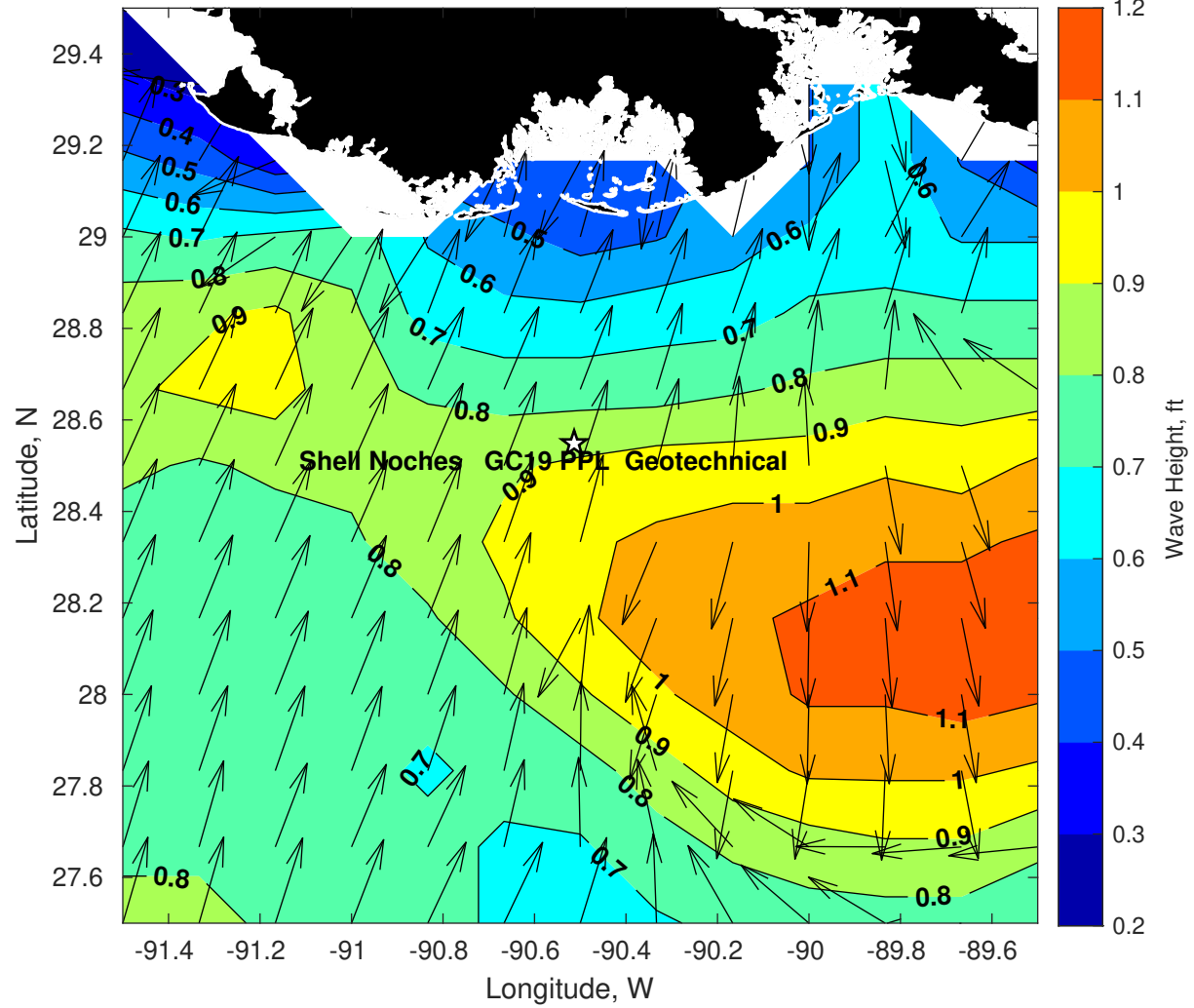
Wave Height (ft) for Shell Noches GC19 PPL Geotechnical at 17-Jul-2025 09:00:00
