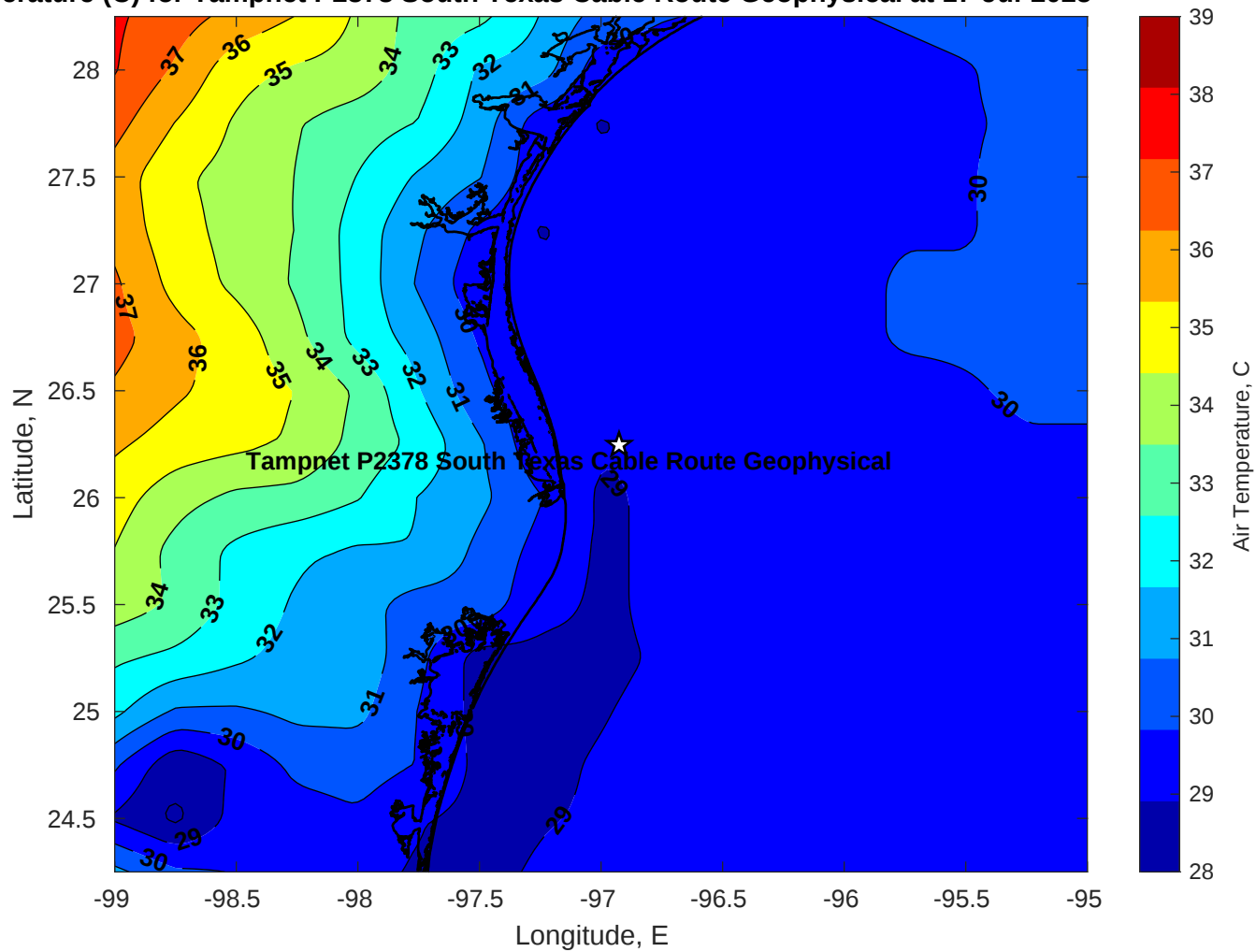
Air Temperature (C) for Tampnet P2378 South Texas Cable Route Geophysical at 17-Jul-2025
