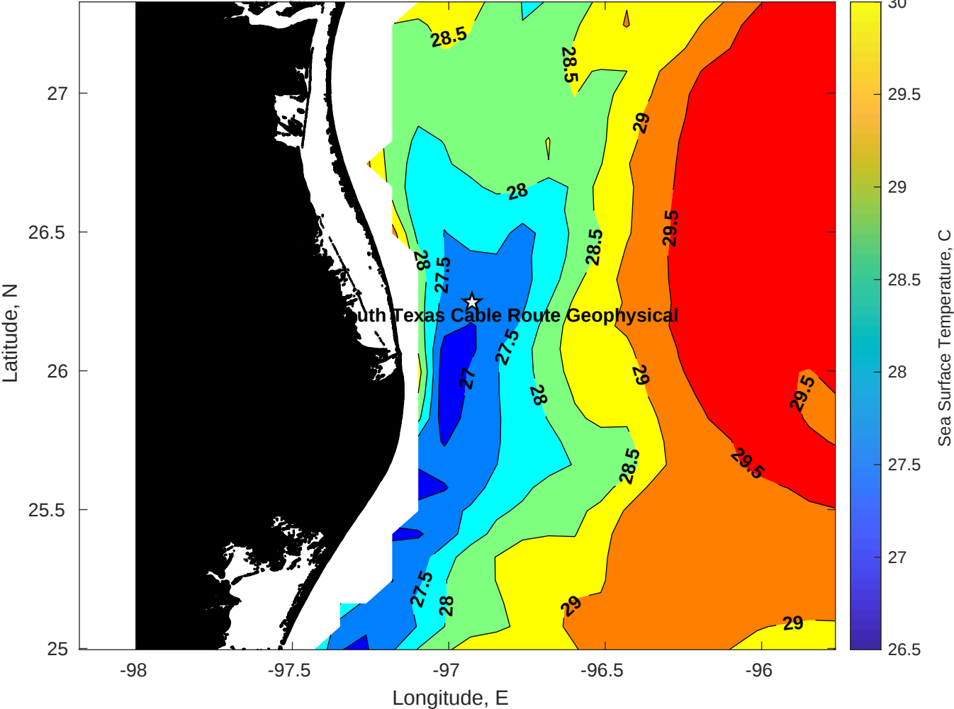
SST for Tampnet P2378 South Texas Cable Route Geophysical at 16-Jul-2025 00:00:00
