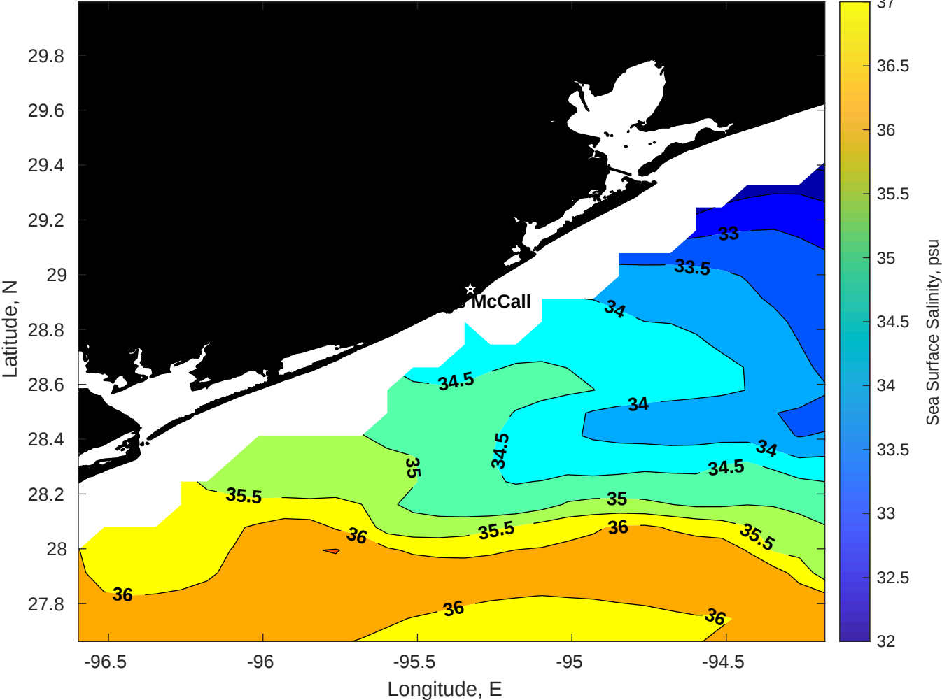
Surface Salinity for Brooks McCall at 17-Jul-2025 00:00:00
