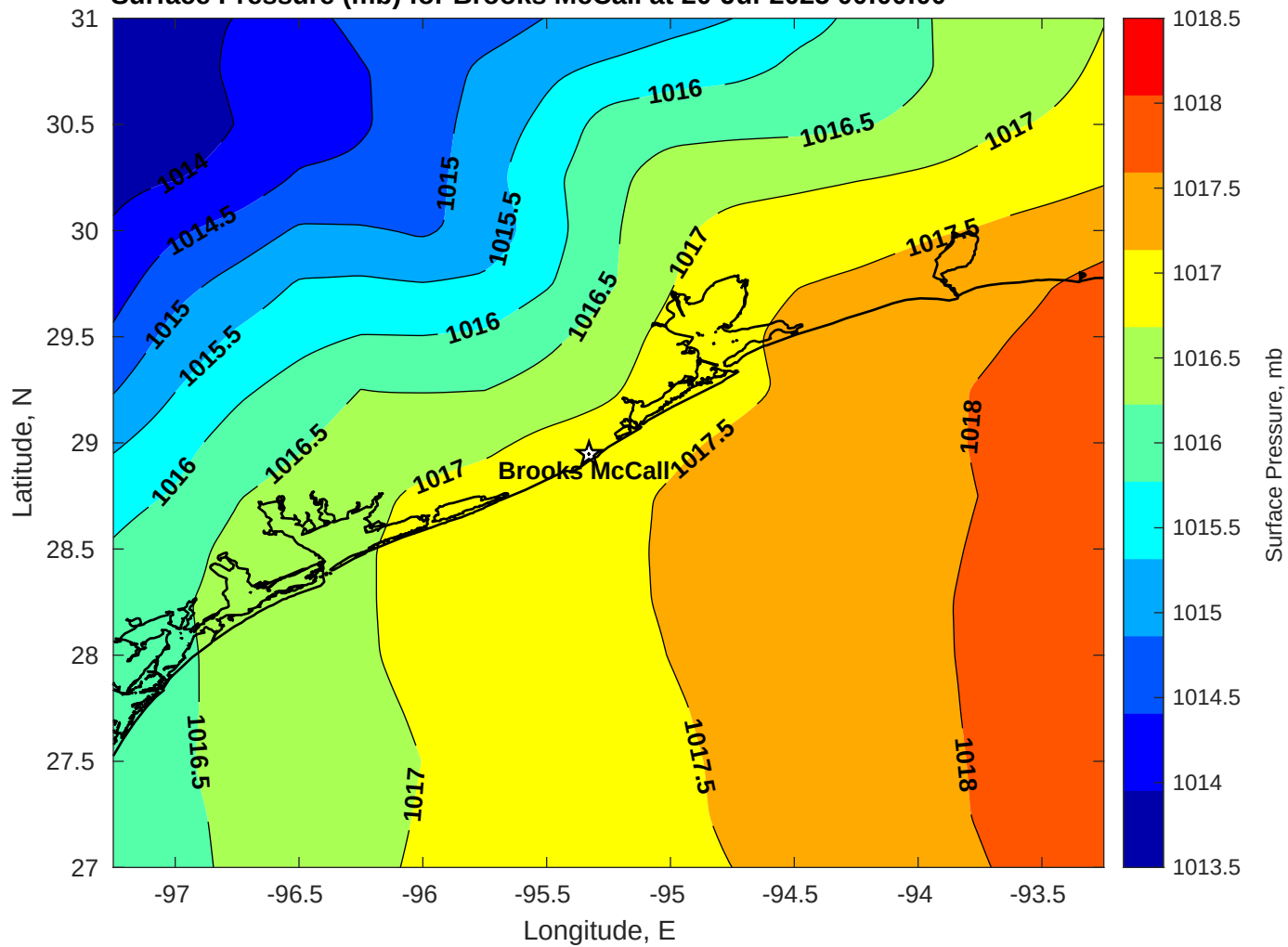
Surface Pressure (mb) for Brooks McCall at 20-Jul-2025 00:00:00
