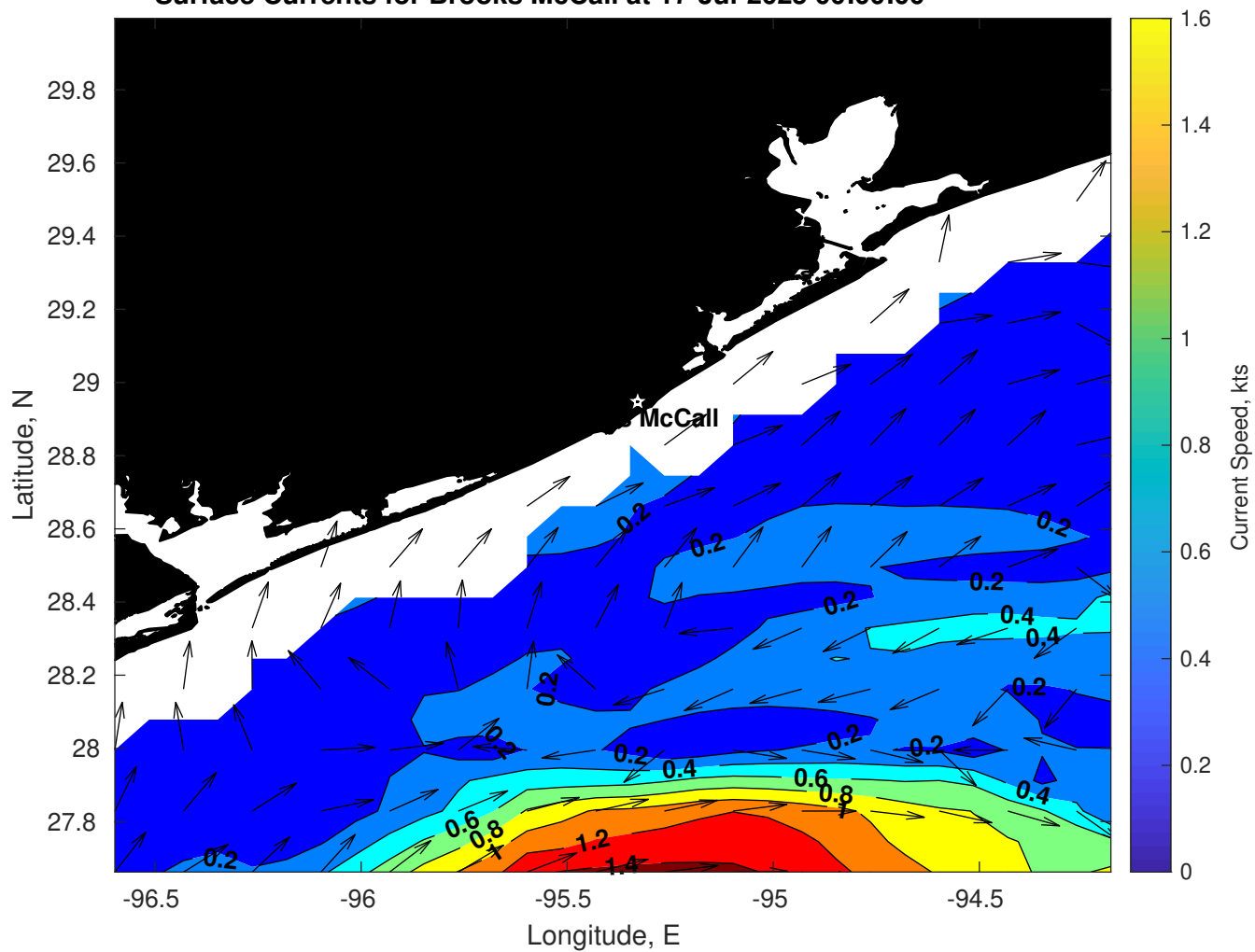
Surface Currents for Brooks McCall at 17-Jul-2025 00:00:00
