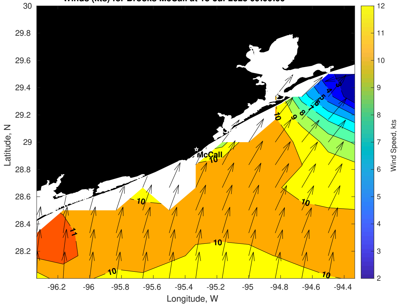
Winds (kts) for Brooks McCall at 18-Jul-2025 09:00:00
