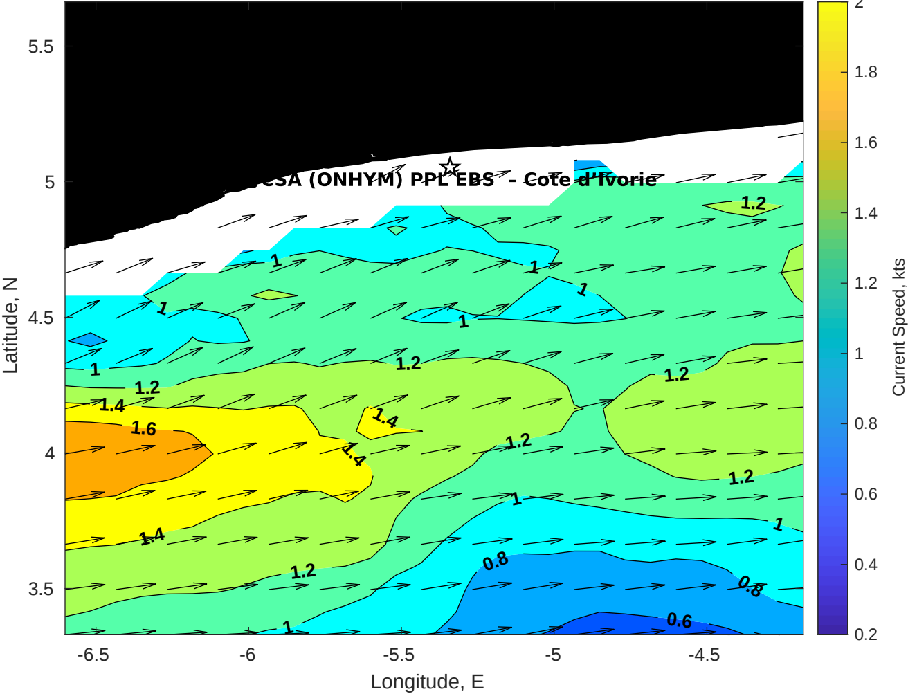
Surface Currents for CSA (ONHYM) PPL EBS - Cote d'Ivoire at 17-Jul-2025 00:00:00
